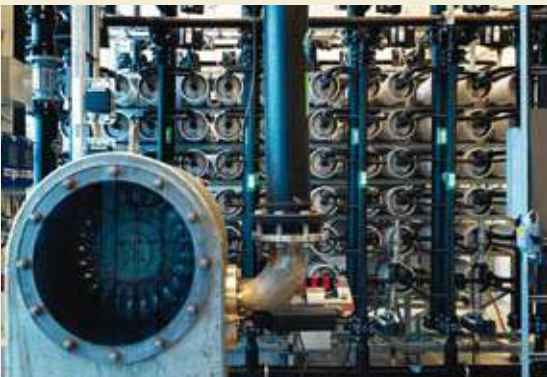
7.12 d > The world's first osmotic power plant on the Oslo Fjord in Norway derives energy from the differences in salt concentration between saltwater and freshwater. A thin membrane separates the water masses, building up pressure which drives a turbine.
