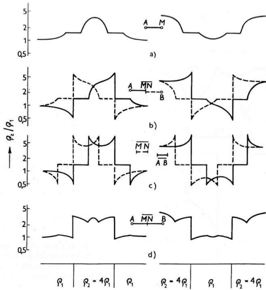
Figure 4.8: Apparent resistivity ( \rho_a ) curves over a thick dyka (Mareš and Tvrđý 1984). a) Potential array. b) Pole-dipole and reversed pole-dipole array. c) Dipole-dipole array. d) Schlumberger array. The reference point (the point at which the measured resistivities are plotted) is in the middle of the potential dipole (or at the potential electrode in case of the potential array).
