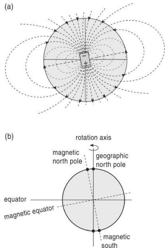
Figure 3.3: Magnetic field of the Earth. (Musset and Khan 2000).
