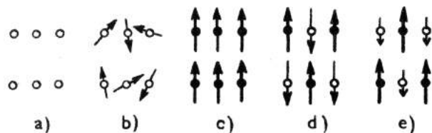
Figure 3.11: Schematic diagram showing orientation of magnetic moments in the crystal lattice of different materials: a) diamagnetic, b) paramagnetic, c) ferromagnetics, d) antiferromagnetics and e) ferrimagnetic (Mareš and Tvrđý 1984).
