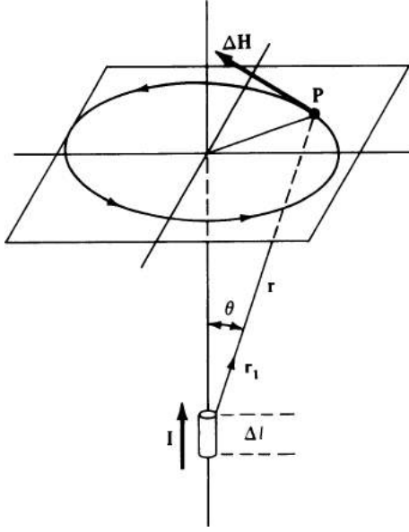
Figure 3.1: Ampère's law. A current I through a length of conductor \Delta l creates a magnetizing field \Delta \mathbf{H} at a point P . (Telford et al. 1990).
