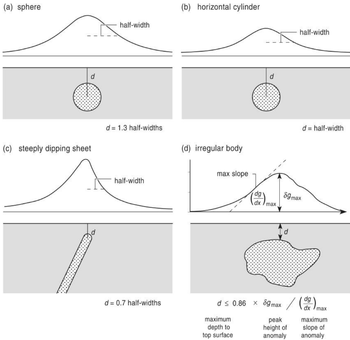
Figure 2.18: Depth rules for various bodies (Musset and Khan 2000).
