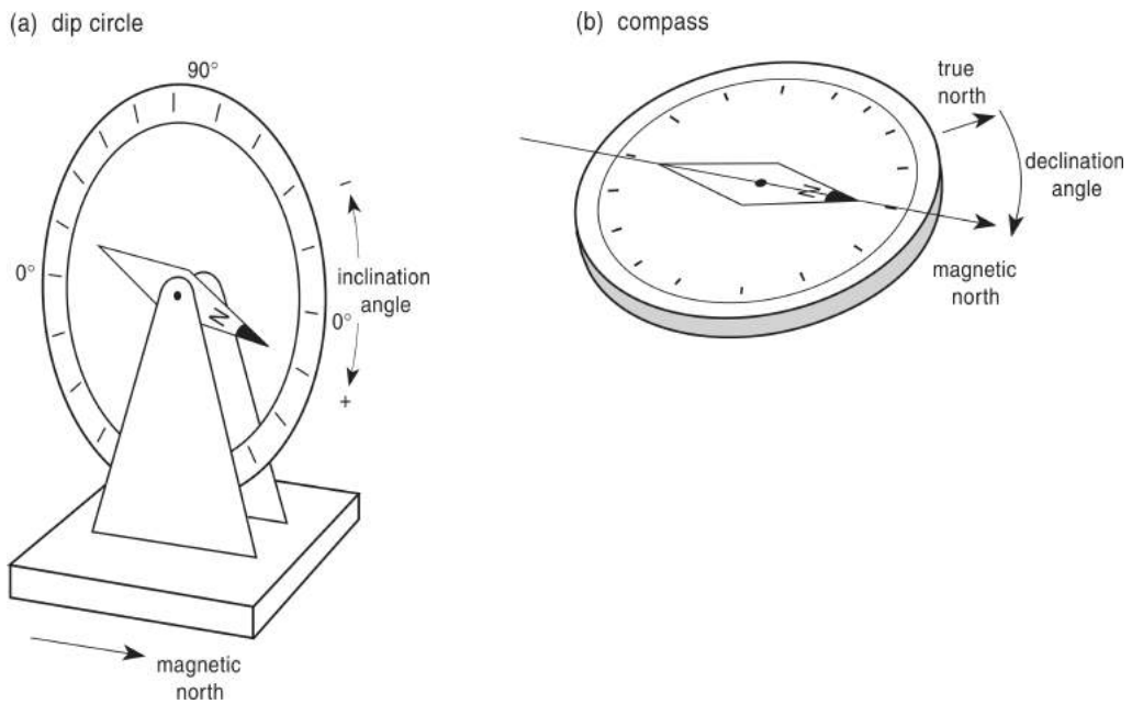
Figure 3.4: Declination and inclination of the Earth's magnetic field. (Musset and Khan 2000).
