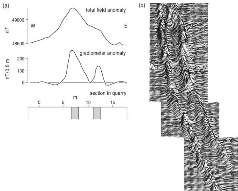
Figure 3.24: Gradiometer survey of the dolerite Butterton dyke, England (Musset and Khan 2000). The total field (a) does not reveal the fact that the dyke is in fact two thin parallel dykes. Nevertheless, this could be clearly recognised from the vertical gradient data. The set of parallel profiles maps a course of the dyke (b).
