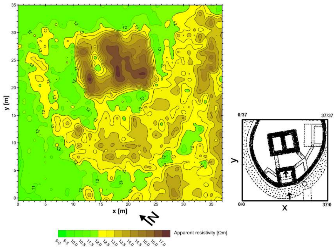
Figure 4.21: Resistivity survey over the former medieval fortress, Czech Republic. Wenner array with a 1 m inter-electrode distances was used, the resistivities were mapped in the 1×1 m grid. The map of apparent resistivities (left) indicates the remnants of masonry as zones with increased resistivities. The interpreted ground-plan (right) shows the central tower, entrance with a gate, fortifications with adjacent smaller buildings and a ditch (dotted).
