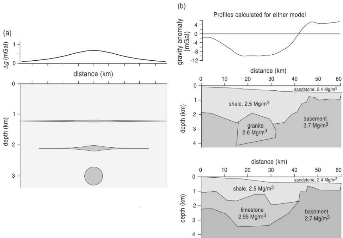
Figure 2.16: Non-uniqueness of the gravity interpretation. The plotted models produce exactly the same gravity anomalies (Musset and Khan 200).
