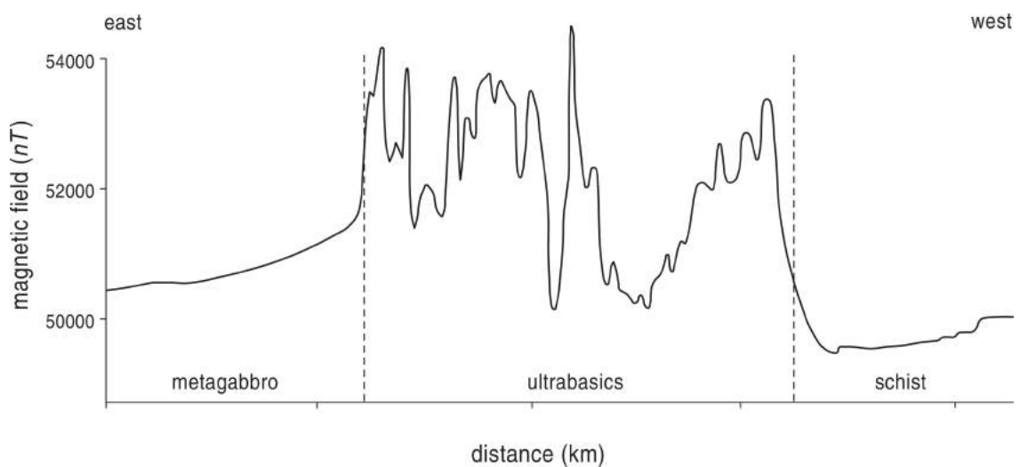
Figure 3.18: Anomaly across geological contacts, Unst, Shetland Islands (Musset and Khan 2000). The ultrabasics are heavily altered, which causes large variations in their magnetization.
