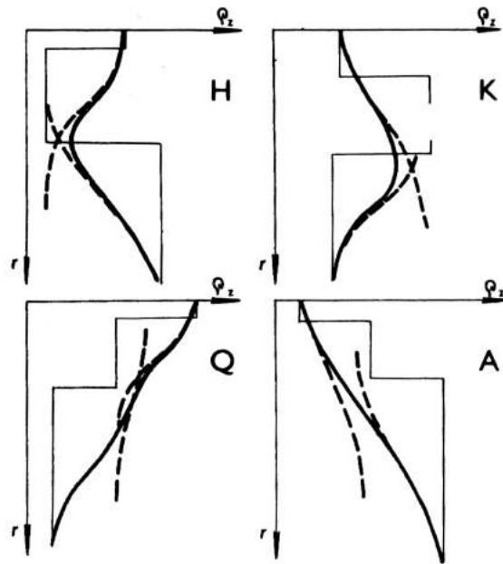
Figure 4.13: The four types of three layer curves and corresponding two layer cases (Mareš and Tordý 1984).
