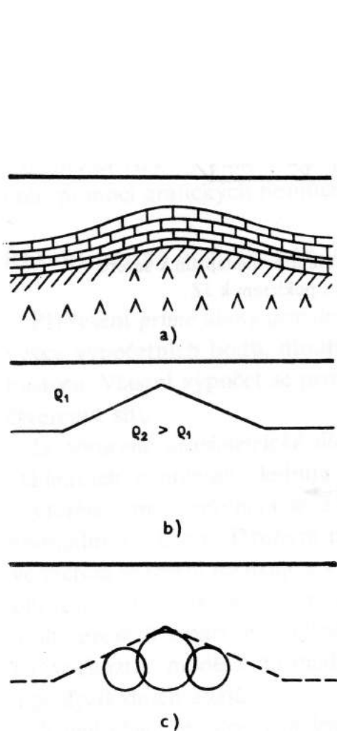
Figure 2.12: Approximation of an anticline (Mareš and Tvrđý 1984). a) A geological section of an anticline. b) A schematic representation with density distribution. c) An approximation of the anticline by three infinite horizontal cylinders.
