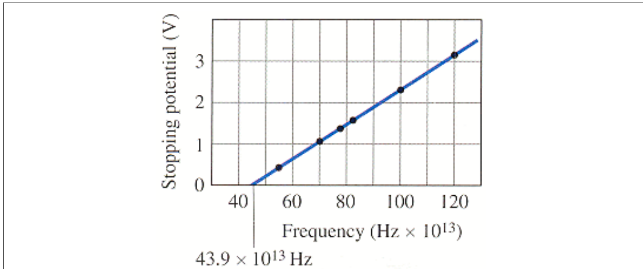
Figure 21: The result of Millikan’s experiment on the photoelectric effect showing the stopping potential against the frequency of incident radiation. The slope, \Delta V/\Delta f is Planck’s constant divided by the electric charge of the electron. The intercept is equal the work function divided by Planck’s constant.
