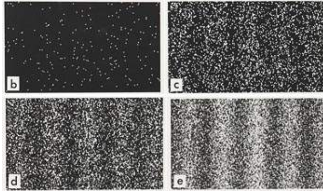
Figure 29: The distribution of the detector-screen of electrons passing individually through a double-slit as time advances. At later times well-defined maxima and minima can be identified.
