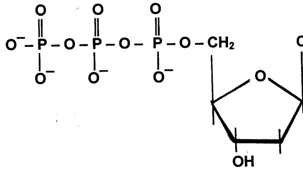
deoxycytidine-5'-triphosphate charge = -4
