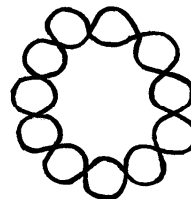
circular
