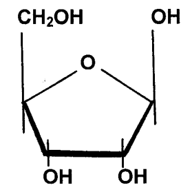
β-D-ribofuranose
