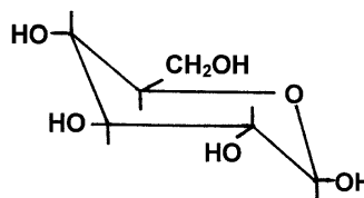
\beta
