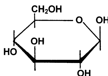
\beta -D-glucopyranose
