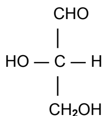
L-glyceraldehyde
