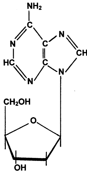
deoxyadenosine
