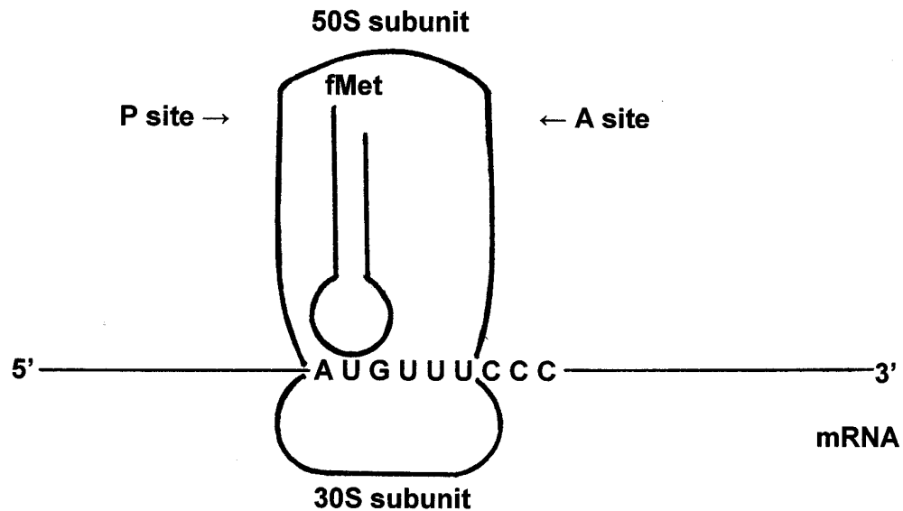
Initiation Complex
