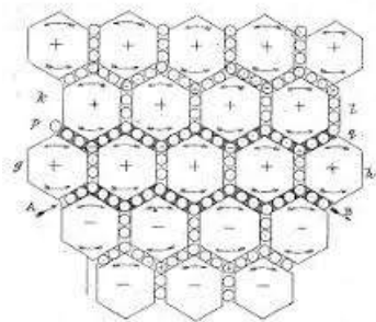
Figure 46: Maxwell's vortices
