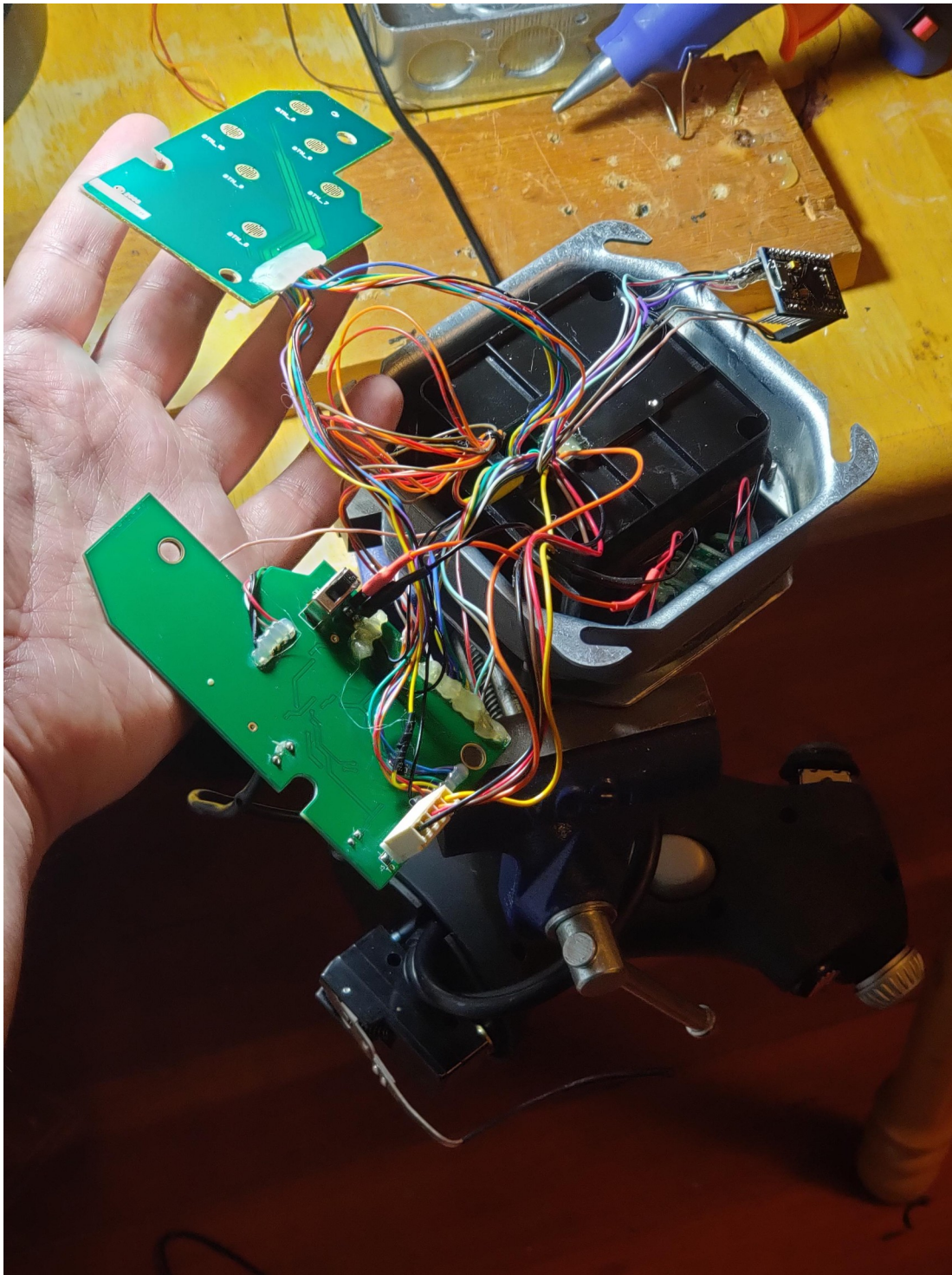
PCBs from the base, now housed in the bottom metal box
