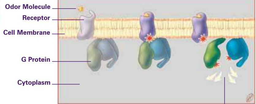
Cascade of Chemical Reactions
