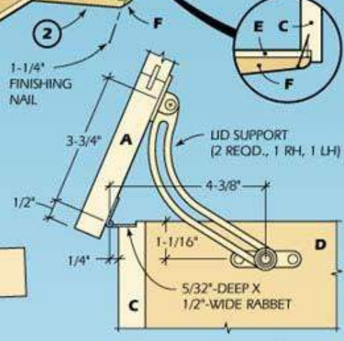
DETAIL 3—LID SUPPORT
