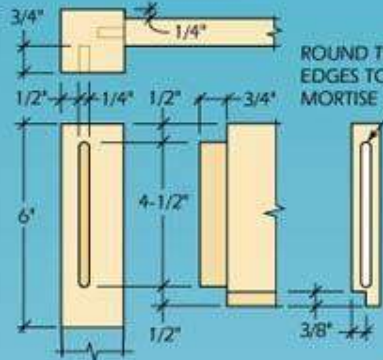
DETAIL 1 TENON AND MORTISE
