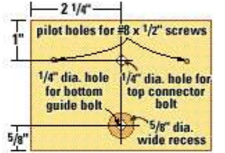
FIXTURE SPACER DETAIL
