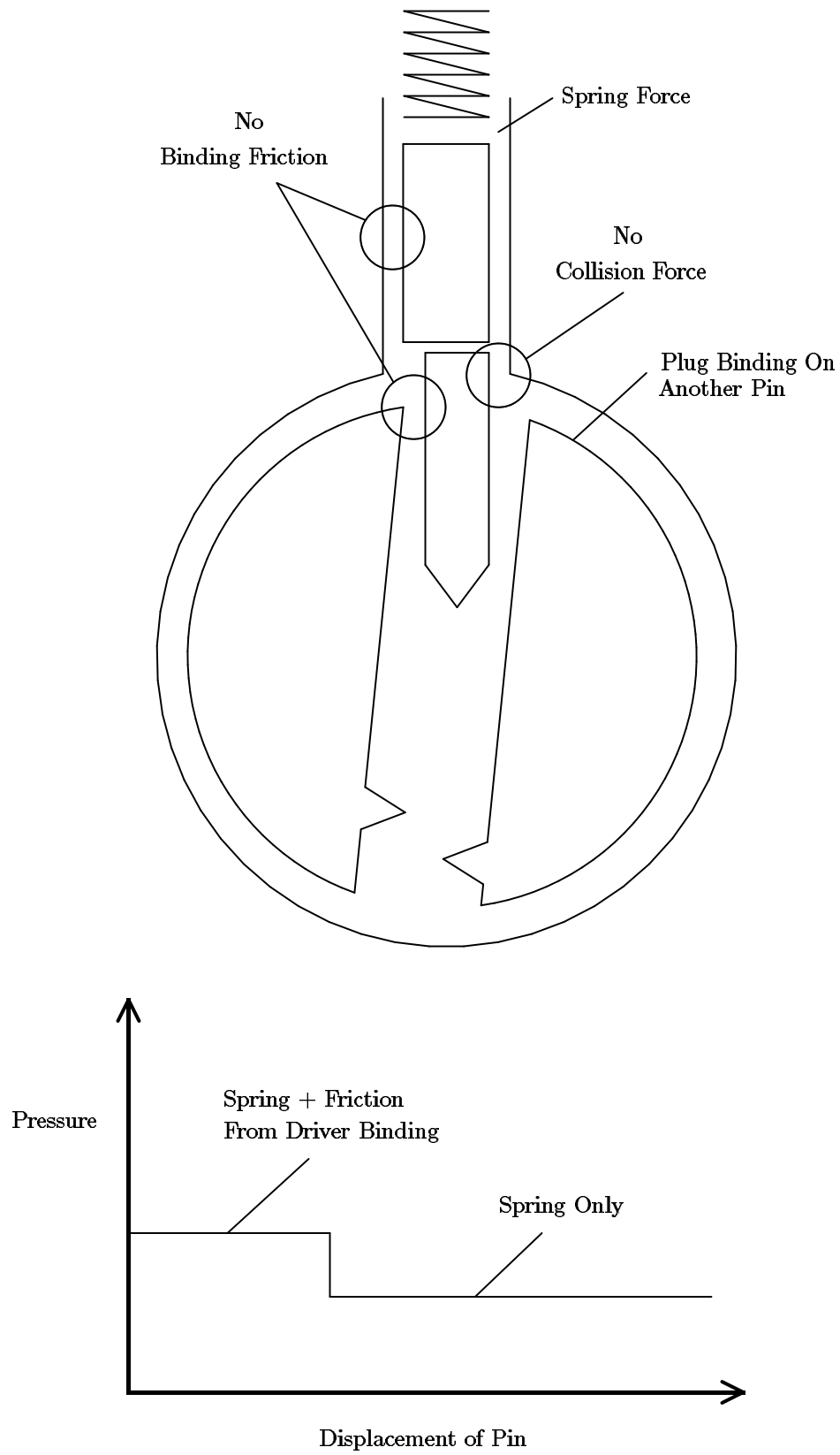
Figure 9.3: Driver pin wider than key pin
