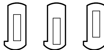
Figure 9.10: Workings of a disk tumbler lock
