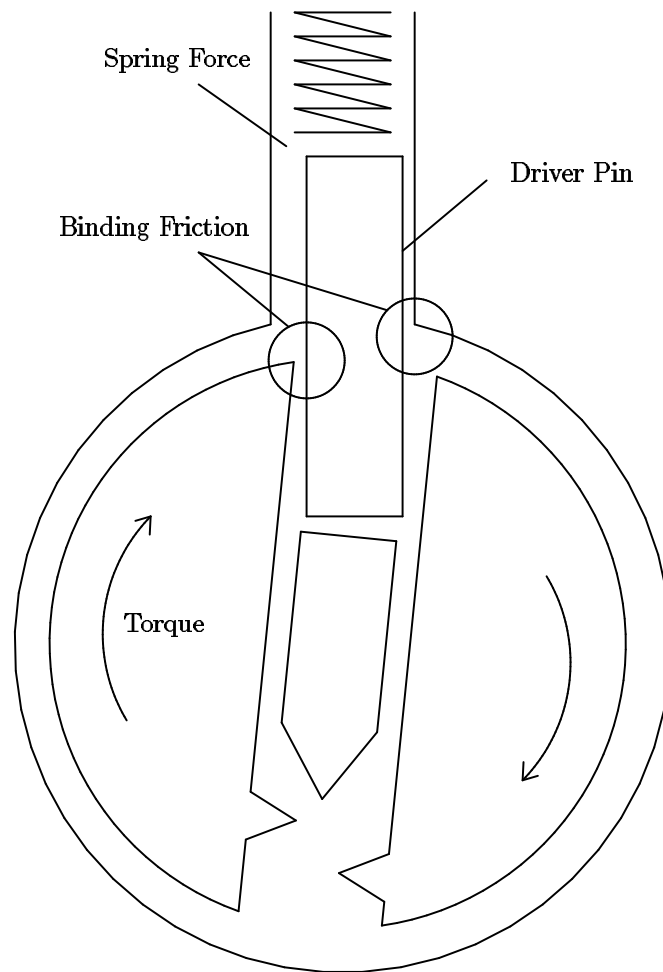
Figure 5.2: Binding in the pin-column model
