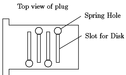
Figure 9.10: Workings of a disk tumbler lock
