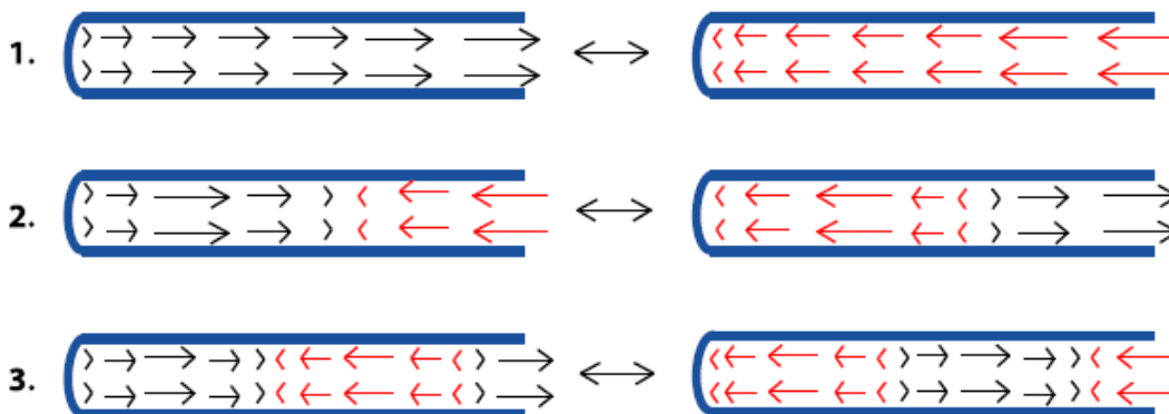
Figure 3.9 Standing Waves in Wind Instruments Standing Waves in a wind instrument are usually shown as displacement waves, with nodes at closed ends where the air cannot move back-and-forth.
