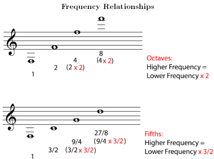
Figure 6.6 Frequency Relationships Remember that, no matter what note you start on, the note one octave higher has 2 times its frequency. Also, no matter what note you start on, the note that is a perfect fifth higher has exactly one and a half times its frequency. Since each of these intervals is so many "times" in terms of frequencies, when you add intervals, you multiply their frequencies. For example, a series of two perfect fifths will give a frequency that is 3/2 \times 3/2 (or 9/4 ) the beginning frequency.
