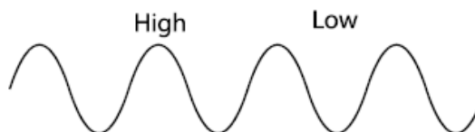
Figure 3.2 Transverse and Longitudinal Waves In water waves and other transverse waves, the ups and downs are in a different direction from the forward movement of the wave. The "high and lows" of sound waves and other longitudinal waves are arranged in the "forward" direction.
