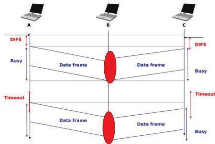
Figure 6.10: Collisions with CSMA/CA
