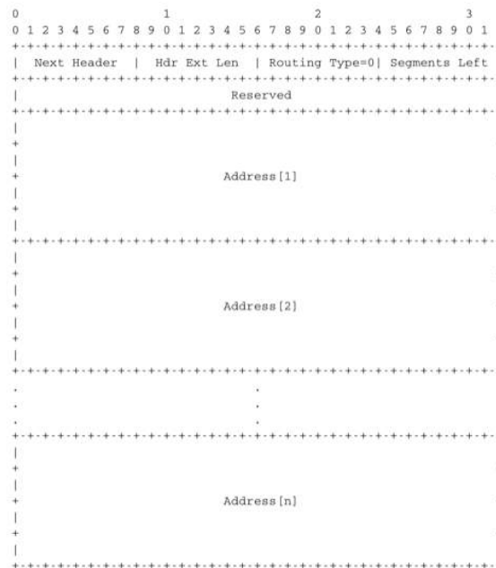
Figure 5.40: The Type 0 routing header ( RFC 2460 )
