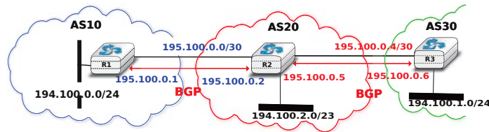
Figure 5.62: Utilisation of the BGP next-hop attribute
