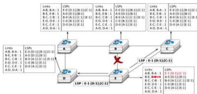
Figure 5.16: The two-way connectivity check
