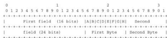
Figure 3.3: Message format
