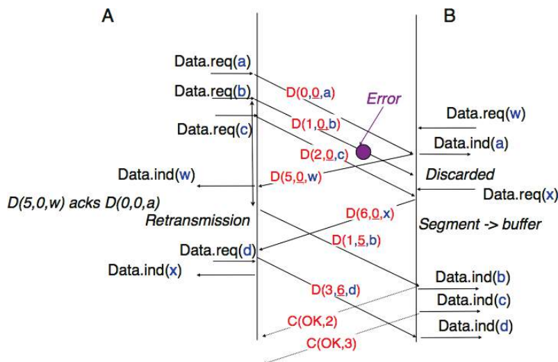
Figure 4.23: Piggybacking
