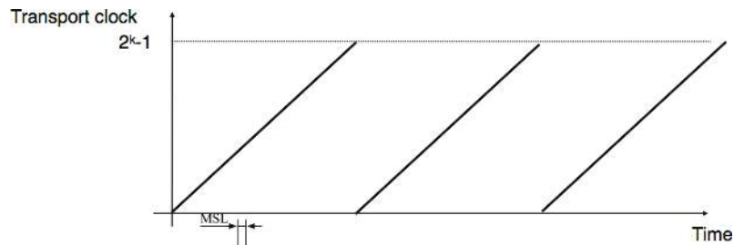
Figure 4.27: Transport clock
