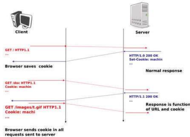
Figure 3.22: HTTP cookies
