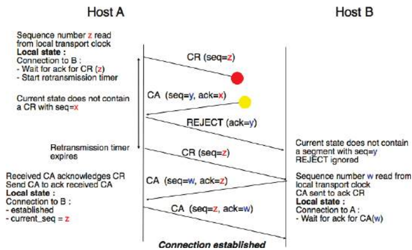
Figure 4.30: Three-way handshake : recovery from a duplicate CA
