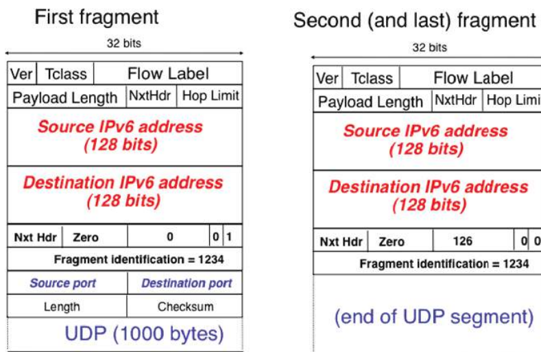
Figure 5.41: IPv6 fragmentation example
