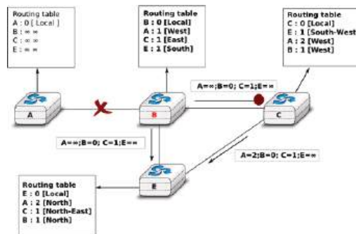
Figure 5.12: Count to infinity problem
