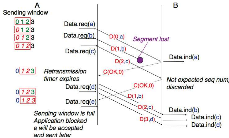
Figure 4.17: Go-back-n : example
