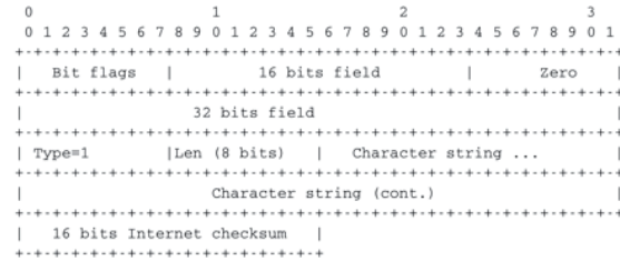
Figure 4.63: Simple SDU format
