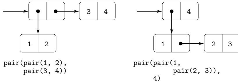
Figure 2.3 Two ways to combine 1, 2, 3, and 4 using pairs.
