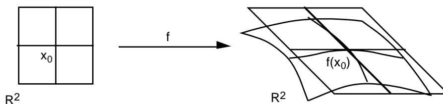
The right curved grid is the image of the left grid under f The right straight grid is the image of the left grid under the first order map x \mapsto f(x_0) + \langle f'(x_0), x - x_0 \rangle
