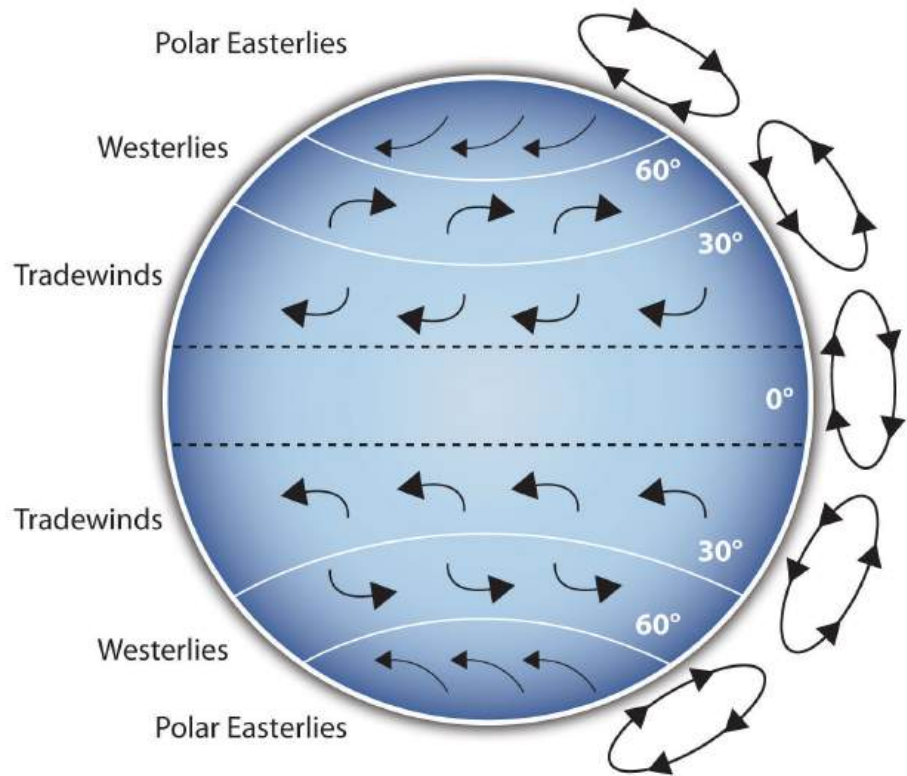
Figure 15.1 Coriolis Effect
