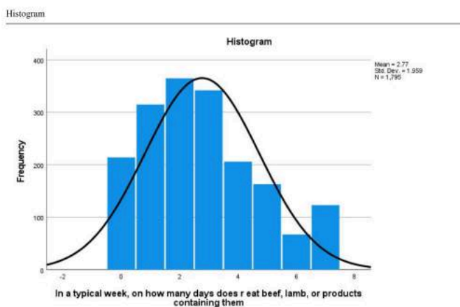
Figure 12. SPSS Output for Descriptive Statistics on EATMEAT
