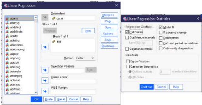
Figure 2. The Linear Regression Dialog
