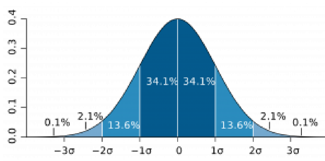
Figure 2.1 The Normal Curve
