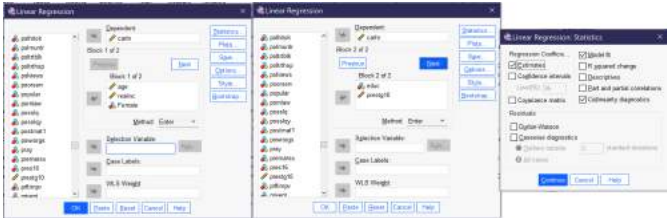
Figure 5. Setting Up a Linear Regression With Blocks
