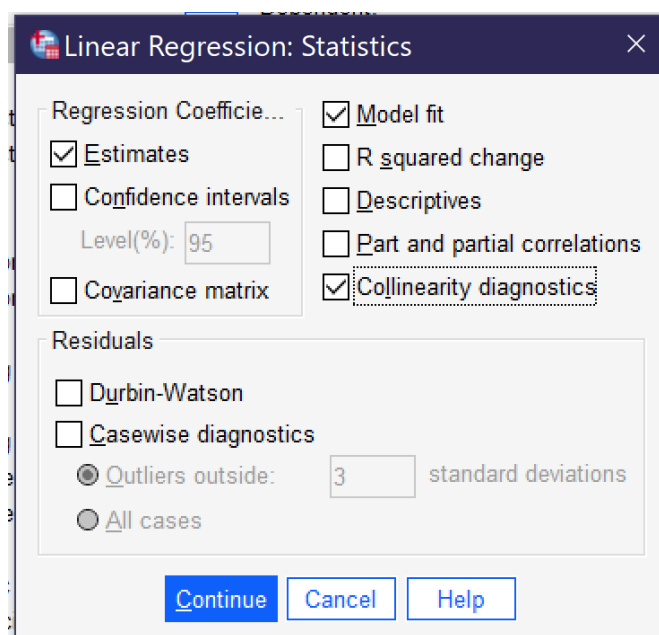
Figure 1. Using Collinearity Diagnostics in Regression
