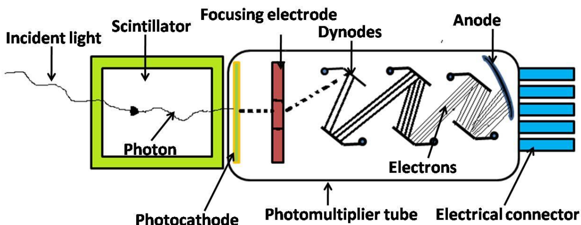
Fig.12.14 Scintillation Counter
