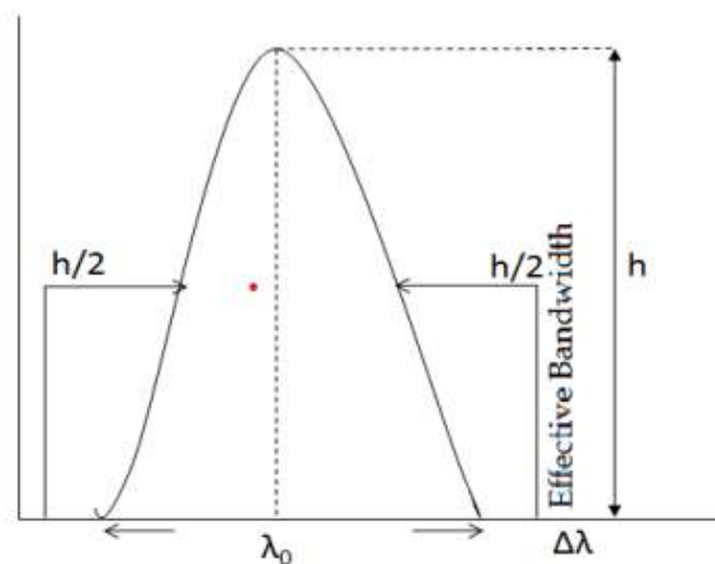
Figure 12.5 Effective Bandwidth
