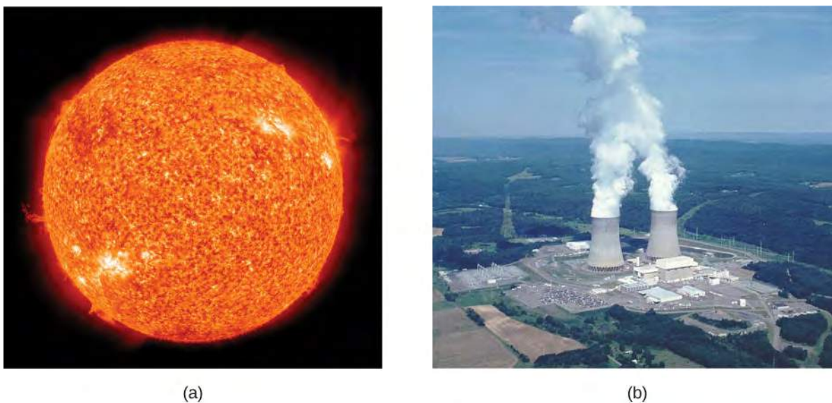
Figure 5.28 (a) The sun and (b) the Susquehanna Steam Electric Station both convert mass into energy—the sun via nuclear fusion, and the electric station via nuclear fission. (credit a: modification of work by NASA/SDO (AIA) )
