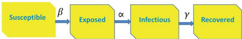
Figure 1. A schematic diagram showing the transmission model for COVID-19 pandemic.
