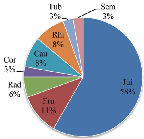
Figure 3. The percentage value of the plant part.
