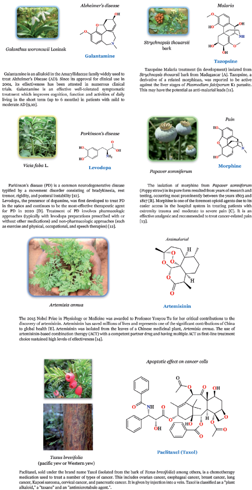
Figure 1. Chemical structures of a few important bioactive compounds isolated from plants.
