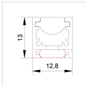
Clip fixing
