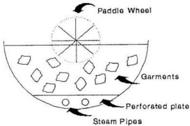
Fig. Paddle dyeing machine.
