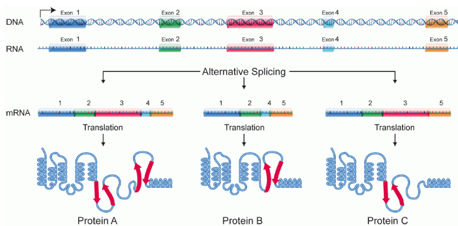
Figure 03-15: Examples of alternative splicing by the National Human Genome Research Institute. Protein A expresses all of the exons. In protein B, exon 3 is skipped, whereas in protein C, exon 4 is skipped. As a result, proteins B and C are each missing a domain. This image is in the public domain.
