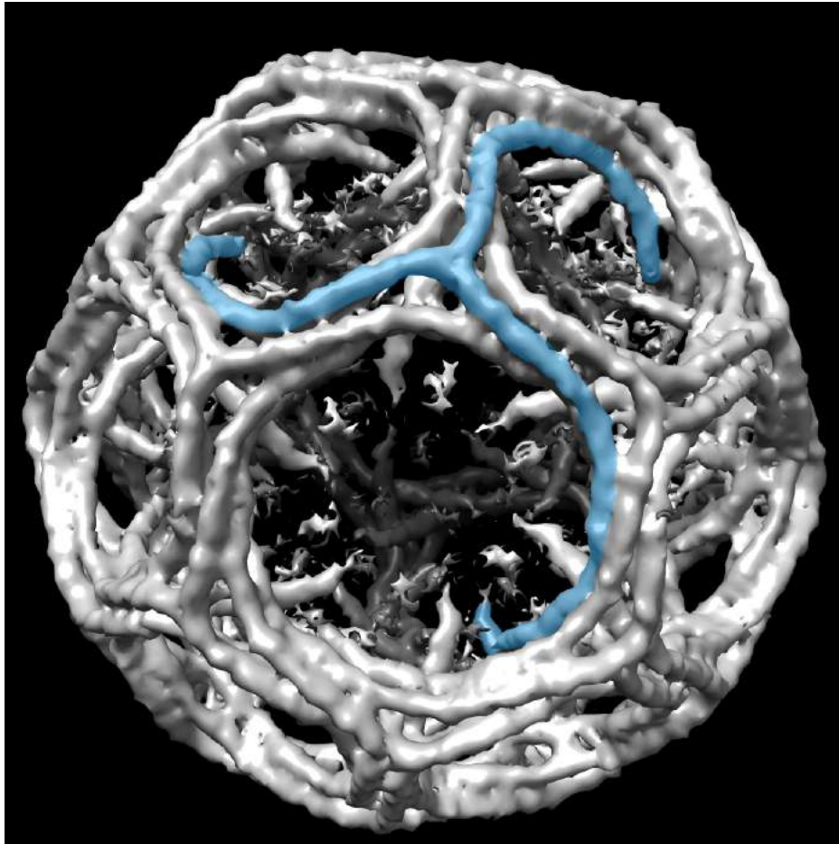
Figure 04-18: Cryo-electron microscopy of clathrin coat. This coat is made of 36 triskelions and is approximately 90 nm in diameter. A single triskelion is highlighted in blue. "Clathrin cage viewed by cryoelectron microscopy" by Mazuraan is shared under a CC BY-SA 4.0 International license.
