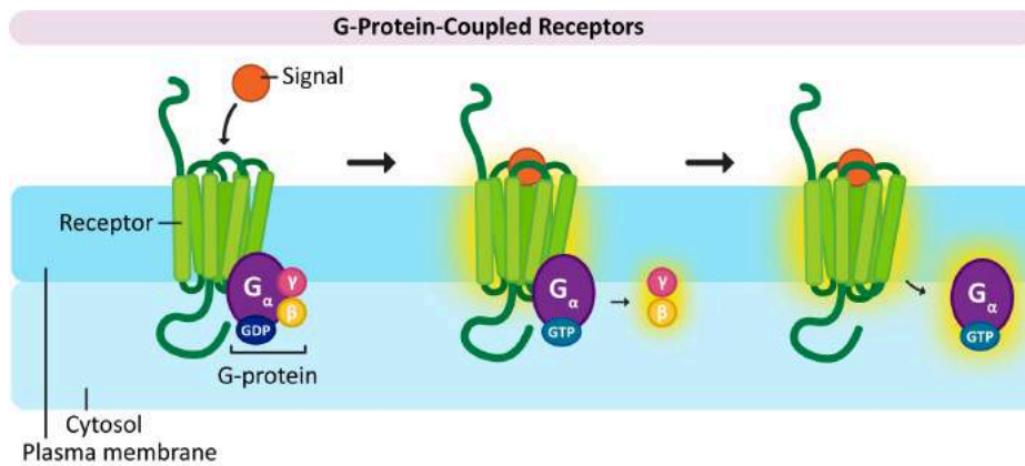
Figure 07-07: The activation of G-proteins. When a signal molecule binds, this activates the G-protein-coupled receptor. The activated receptor swaps out GDP for GTP on G_\alpha . When bound to GTP, the G_\alpha separates from G\beta\gamma . These two molecules stimulate further downstream signaling. This image was created by Heather Ng-Cornish and is shared under a CC BY-SA 4.0 license.
