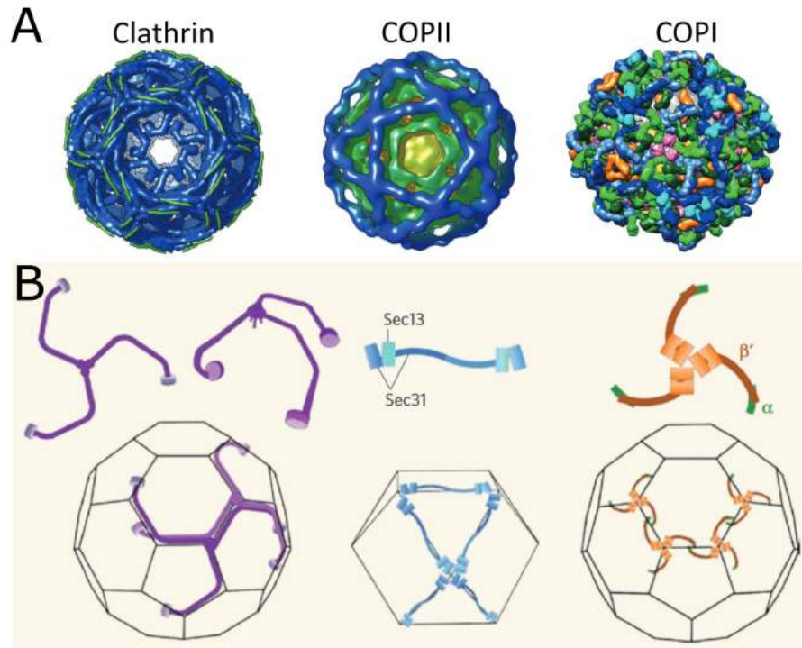
Figure 04-19: Molecular structure of the different coat proteins. (A) Molecular models from Noble and Stagg (2015). (B) Schematic coat proteins overlaying a sketched cage structure from Harrison and Kirchhausen (2010). Average diameters for all vesicle coats shown are roughly similar, ranging from 60 nm (COPI) and 90 nm (clathrin), with COPII somewhere in the middle. Panel (A) is from Noble, A. J., & Stagg, S. M. (2015). COPI gets a fancy new coat: An interconnected scaffolding of proteins bends the membrane to form vesicles. Science , Volume 349, Issue 6244, July 2015, Pages 142–143. http://www.jstor.org/stable/24748469 . Reprinted with permission from AAAS. Please do not redistribute without permission of the rights holder. Panel (B) is included under fair use as described in the CBPFUOER. Please do not redistribute without permission of the rights holder.
