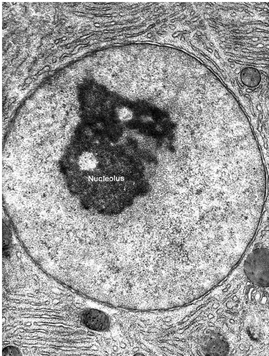
Figure 03-22: Electron micrograph of the nucleolus in a pancreatic acinar cell. Original image from the Cell Image Library, Don W. Fawcett (2011), CIL:10974. Dataset. https://doi.org/10.7295/W9CIL10974 . CC-BY-NC-ND 3.0 license.
