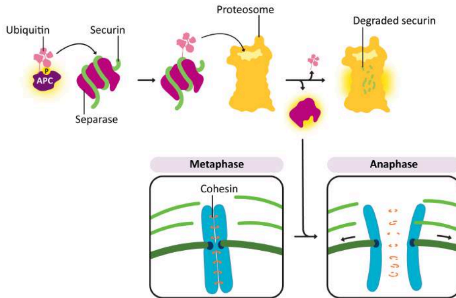
Figure 08-16: The anaphase-promoting complex (APC) adds ubiquitin to a protein called securin. This marks the protein for degradation. Once securin is removed, separase is active and cleaves cohesins that hold the sister chromatids together. This results in the separation of the sister chromatids during anaphase. This image was created by Heather Ng-Cornish and is shared under a CC BY-SA 4.0 license.
