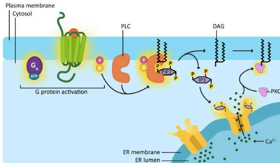
Figure 07-11: Production of second messengers IP _3 and DAG by GPCR activation resulting in the release of calcium ions from the ER lumen. In this image, the lipid tails can be observed as zigzags. This image was created by Heather Ng-Cornish and is shared under a CC BY-SA 4.0 license.
