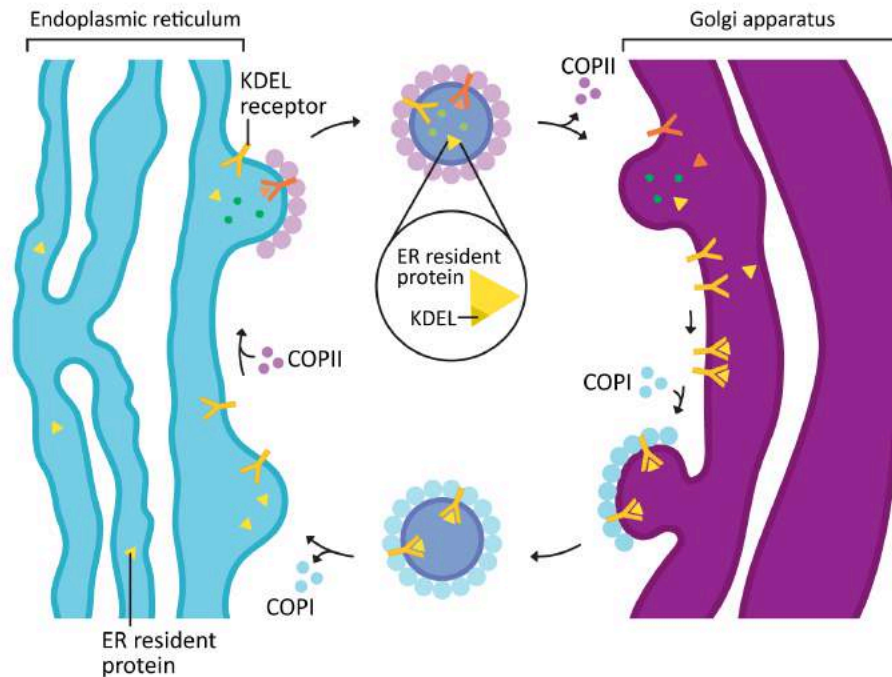
Figure 04-20: Traffic between the ER and Golgi is managed by COPI- and COPII-coated vesicles. Proteins bound for the Golgi are packaged into COPII-coated vesicles. On occasion, ER resident proteins also get trafficked to the Golgi, where they are recognized by the KDEL amino acid sequence and packaged into COPI vesicles that return to the ER. This image was created by Heather Ng-Cornish and is shared under a CC BY-SA 4.0 license.
