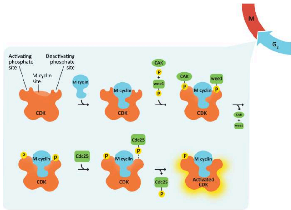
Figure 08-05: The activation of the cyclin-CDK complex by both the addition of phosphate at an activating site and the loss of a phosphate at an inhibitory site. This image was created by Heather Ng-Cornish and is shared under a CC BY-SA 4.0 license.
