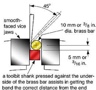
Figure 142 – bending in the vice
