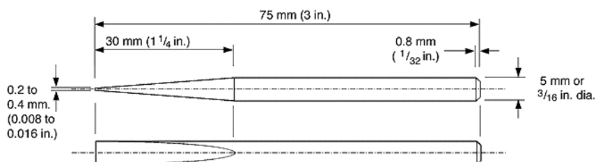
Figure 139 – hand removing levers before bending tip
