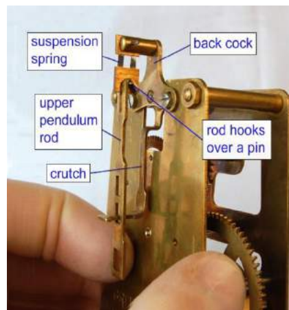
Figure 65 – mounting the pendulum
