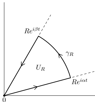
Figura 4.15: Camino \Gamma_R
