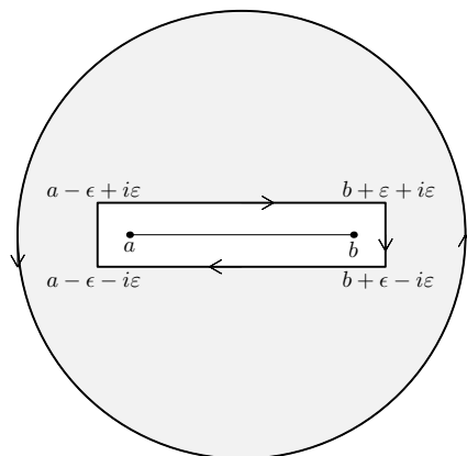
Figura 4.10: \Gamma(R, \varepsilon)
