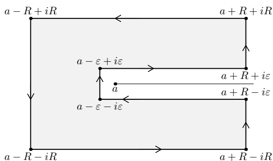
Figura 4.8: \Gamma(R, \varepsilon)
