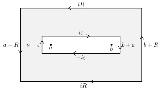
Figura 4.6: \Gamma(R, \varepsilon)
