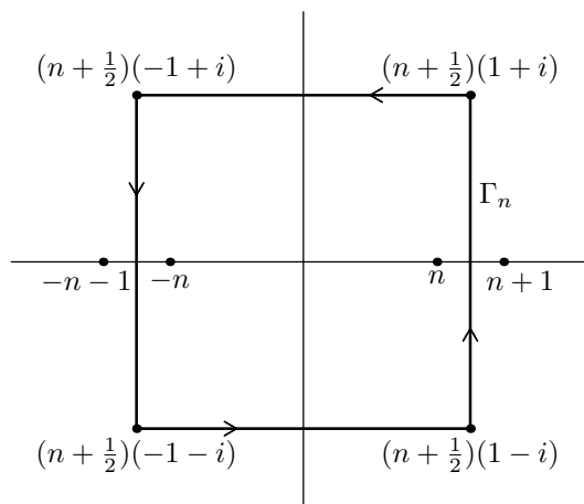
Figura 4.14: Camino \Gamma_n
