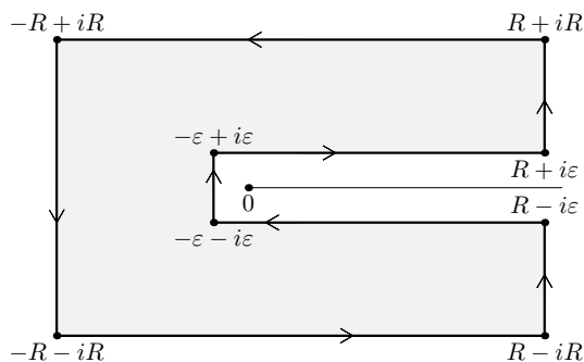
Figura 4.9: \Gamma(R, \varepsilon)
