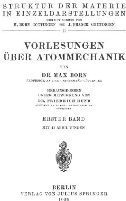
Figure 8.1: Cover page.
