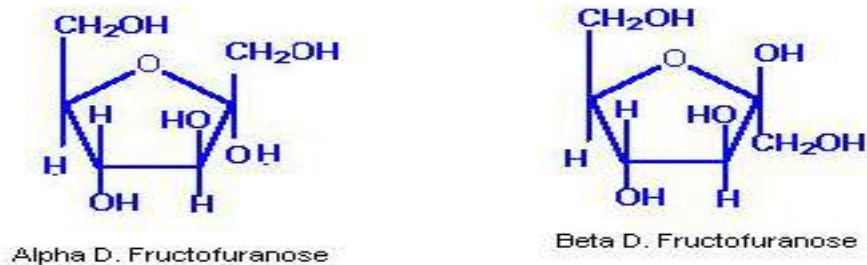
Fig 2.4. \alpha and \beta forms of Fructose
