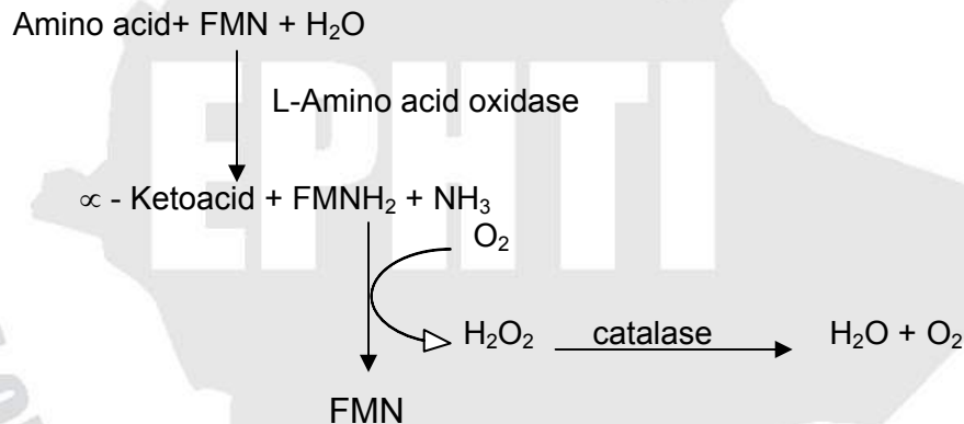
Fig 5.24: oxidative deamination of Amino acids
