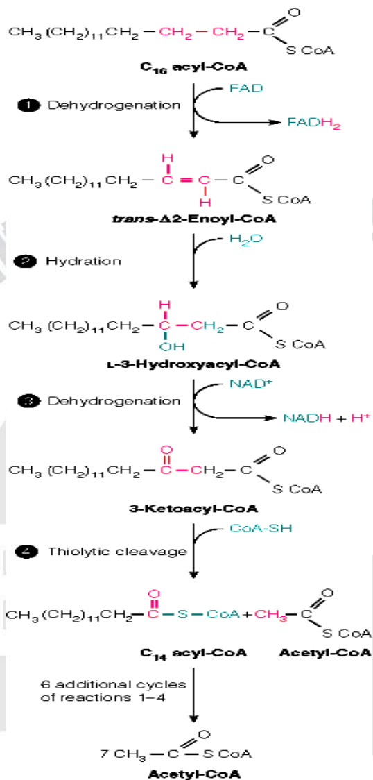
Fig 4.7: β-oxidation of fatty acid
