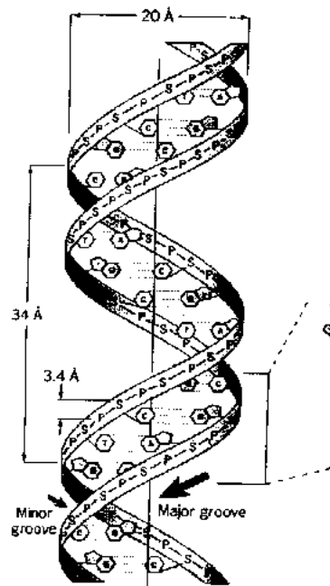
Fig 8.6 secondary structure of DNA
