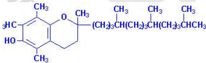
Fig.6.4 Structure of Vitamin E
