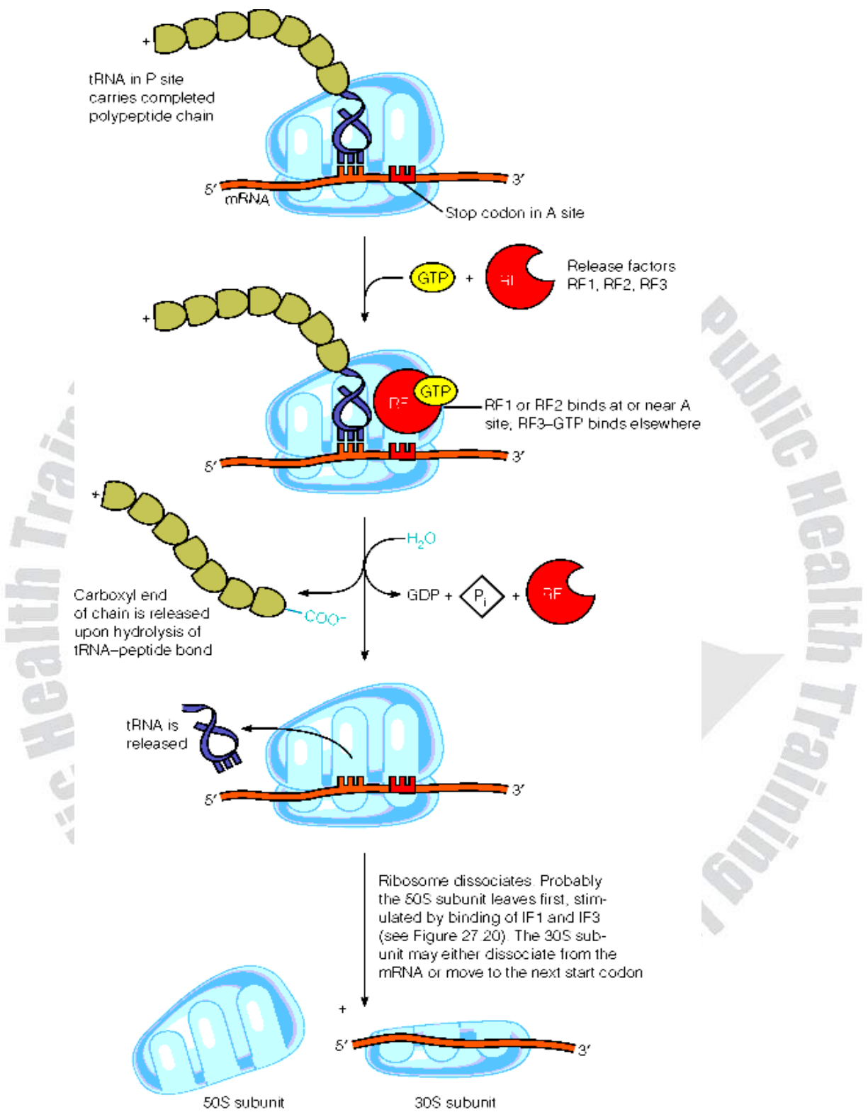
Fig:8.18 Termination of protein synthesis
