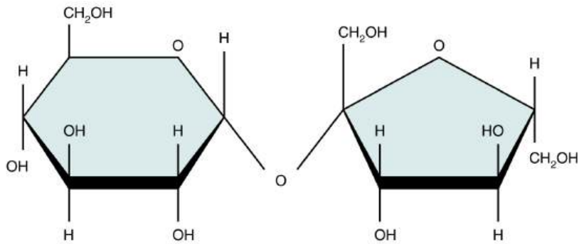
Sucrose
