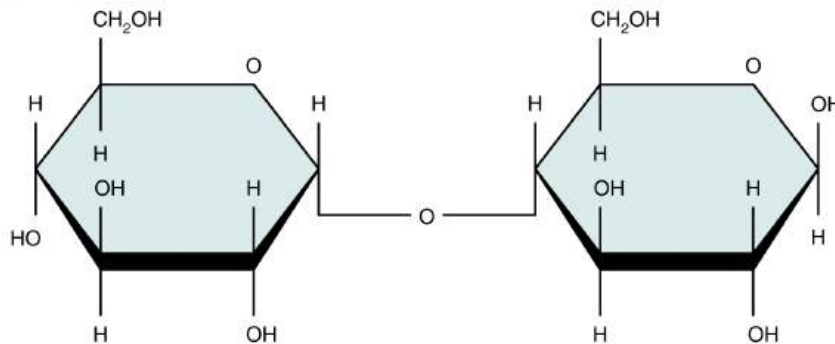
Maltose
