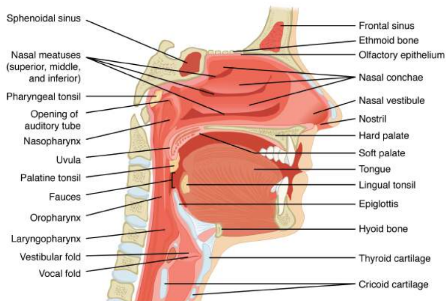
FIGURE 22.4 Upper Airway
