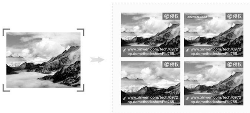
Fig. 1.14 Image search
