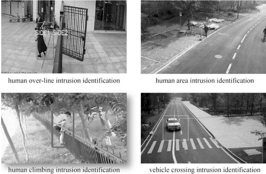
Fig. 8.30 Intrusion identification
