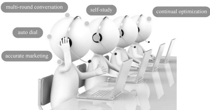
Fig. 8.9 Conversational bot
