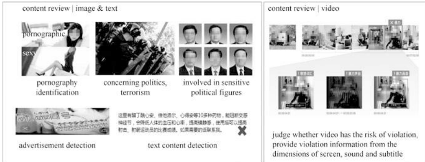
Fig. 8.14 Content review
