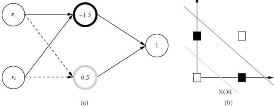
Fig. 3.7 Multilayer perceptron solving the XOR problem
