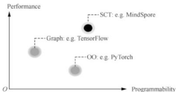
Fig. 5.4 Comparison of automatic differentiation performance and programmability
