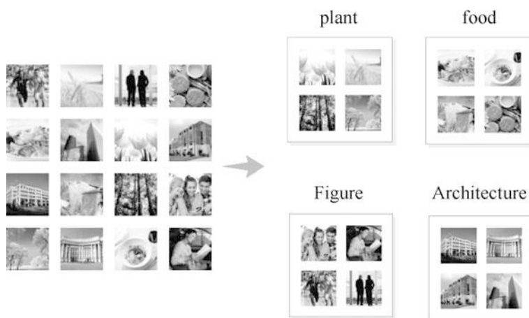
Fig. 1.13 Image recognition
