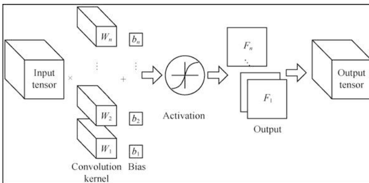
Fig. 3.23 The structure of convolutional layer
