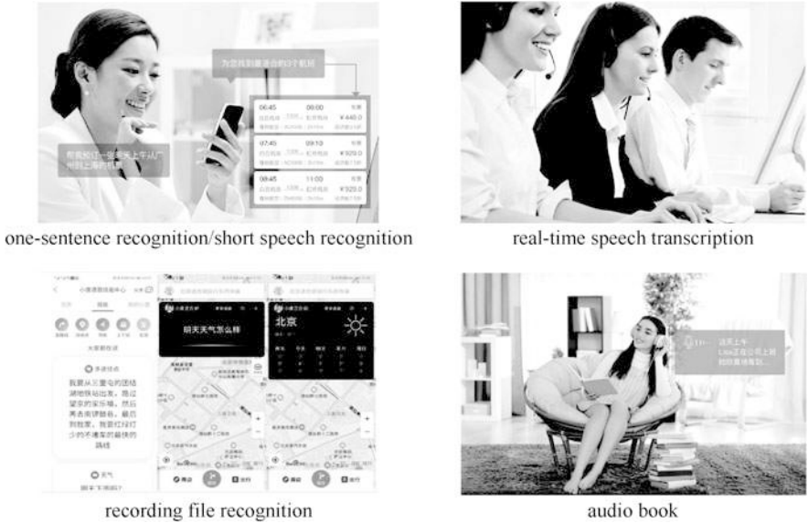
Fig. 8.11 Speech interaction
