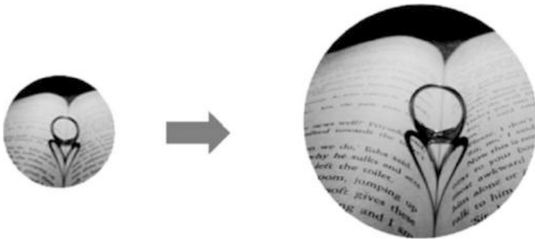
Fig. 7.15 Text super-resolution
