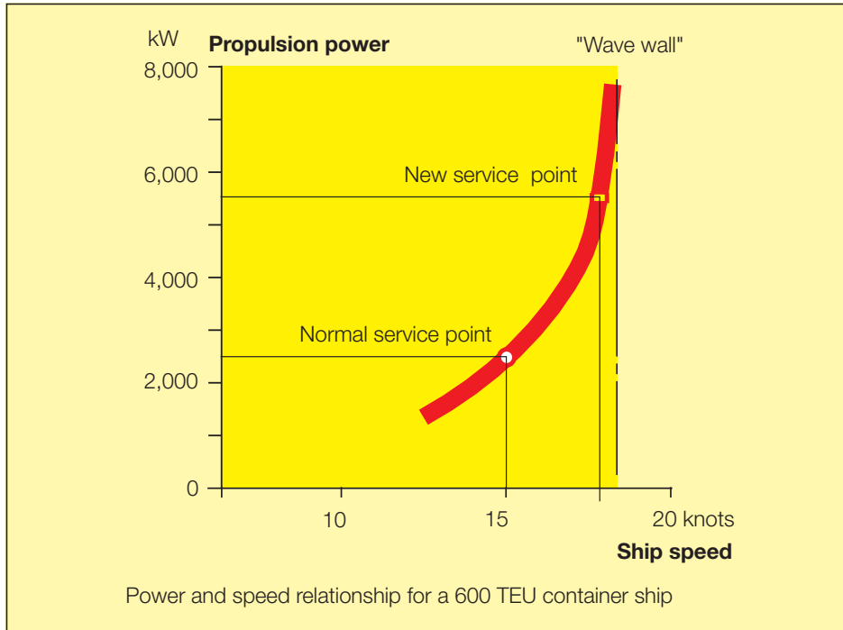
Fig. 5: The “wave wall” ship speed barrier
