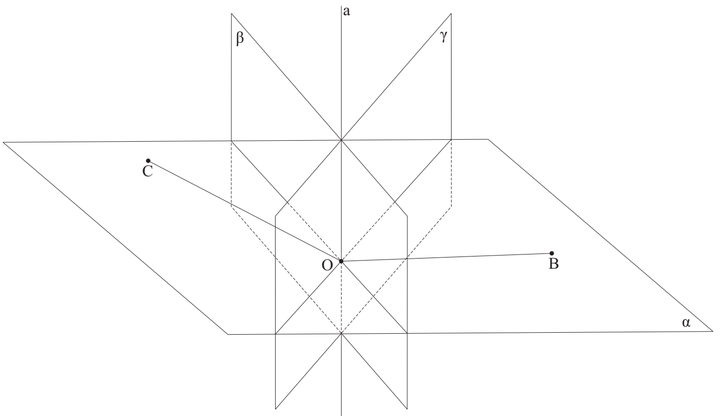
Figure 1.164: Illustration for proof of existence in T 1.3.44.
