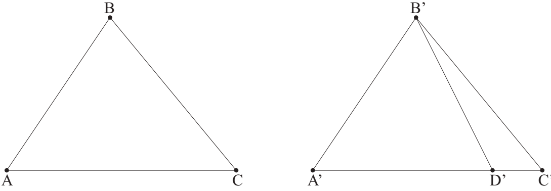
Figure 1.134: If a side AB and angles \angle A , \angle C of a triangle \triangle ABC are congruent, respectively, to a side A'B' and angles \angle A' , \angle C' of a triangle \triangle A'B'C' , the triangles \triangle ABC , \triangle A'B'C' are congruent. (SAA, or The Fourth Triangle Congruence Theorem)
