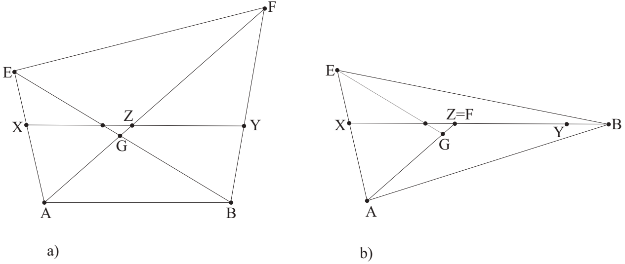
Figure 1.67: Illustration for proof of T 1.2.41.
