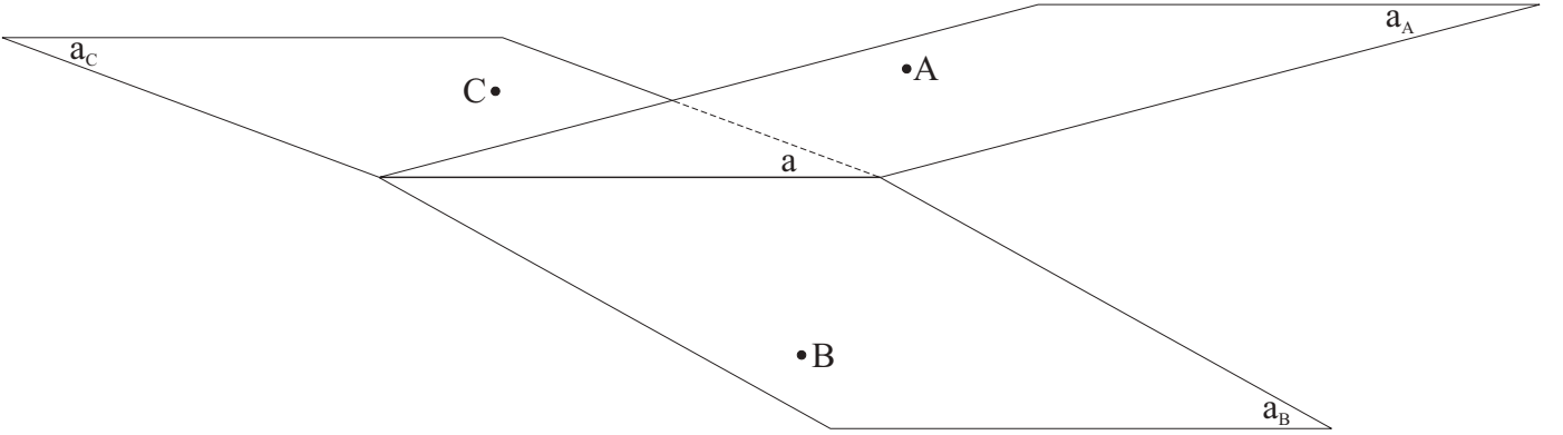
Figure 1.84: If a point C lies outside a dihedral angle \widehat{AaB} , the half-plane a_C lies completely outside \widehat{AaB} : a_C \subset \text{Ext}(\widehat{AaB}) .
