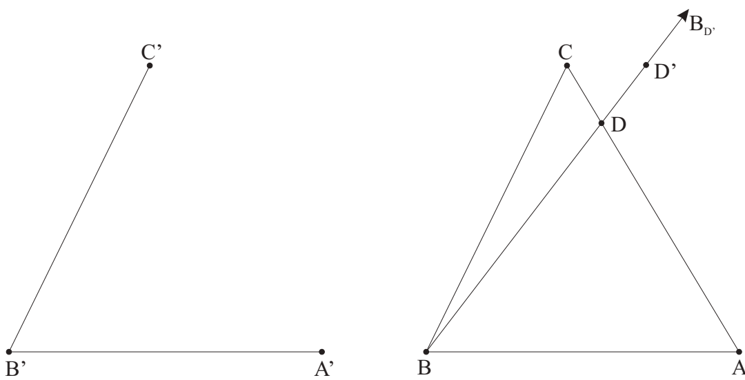
Figure 1.125: If an angle \angle A'B'C' is less than an angle \angle ABC , there is a point D lying between A and C and such that \angle A'B'C' \equiv ABD .
