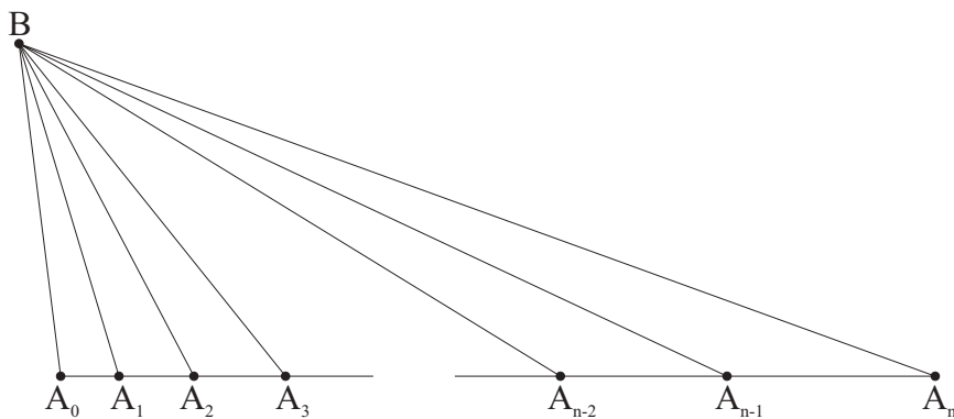
Figure 1.129: Illustration for proofs of C 1.3.18.4, C 1.3.18.5.
