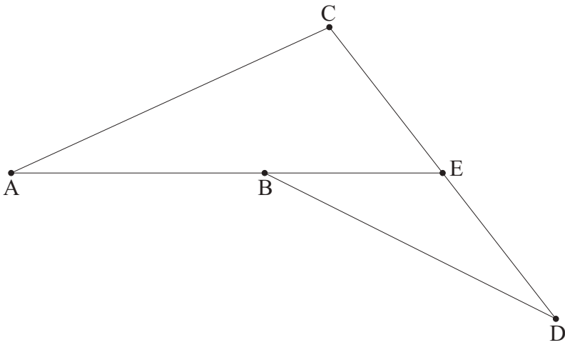
Figure 1.138: Illustration for proof of T 1.3.22.
