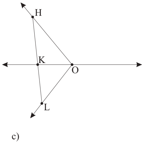
Figure 1.55: Suppose that the rays h , k , l have the same initial point O and the rays h , l lie on opposite sides of the line \bar{k} . Then either k lies inside \angle(h, l) , or k^c lies inside \angle(h, l) , or l = h^c .
