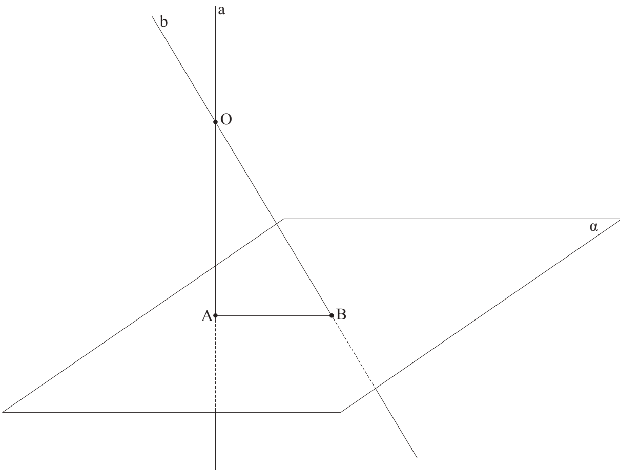
Figure 1.166: Illustration for proof of uniqueness in T 1.3.45.
