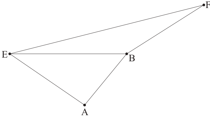
Figure 1.66: If points A, F lie on opposite sides of a line a_{EB} , the quadrilateral FEAB is semisimple.
