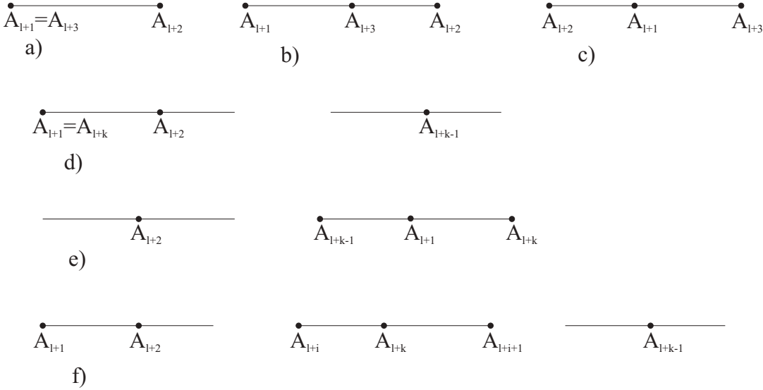
Figure 1.65: Illustration for proof of L 1.2.38.3.
