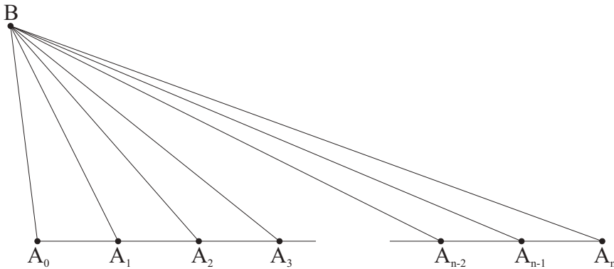
Figure 1.131: Let an interval A_0A_n , n \geq 2 , be divided into n congruent intervals A_0A_1, A_1A_2, \dots, A_{n-1}A_n . Suppose further that B is such a point that \angle BA_0A_1 is greater than \angle BA_1A_0 . Then we have: \angle A_nBA_{n-1} < \angle A_{n-1}BA_{n-2} < \dots < \angle A_3BA_2 < \angle A_2BA_1 < \angle A_1BA_0 .
