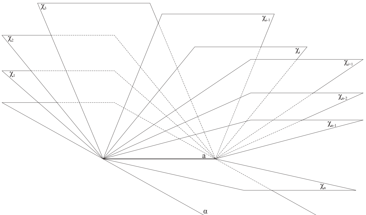
Figure 1.100: Suppose \chi_1, \chi_2, \dots, \chi_n, (\dots) is a finite (countably infinite) sequence of half-planes of the pencil \mathfrak{J} with the property that a half-plane of the sequence lies between two other half-planes of the sequence if its number has an intermediate value between the numbers of these half-planes. Then the converse of this property is true, namely, that if a half-plane of the sequence lies inside the dihedral angle formed by two other half-planes of the sequence, its number has an intermediate value between the numbers of these two half-planes.
