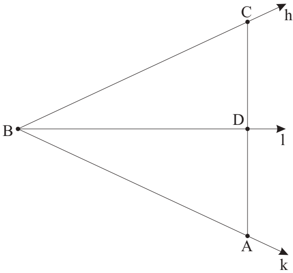
Figure 1.143: Every angle \angle(h, k) has a unique bisector l .
