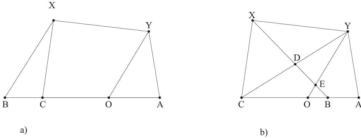
Figure 1.74: Illustration for proof of T 1.2.48.
