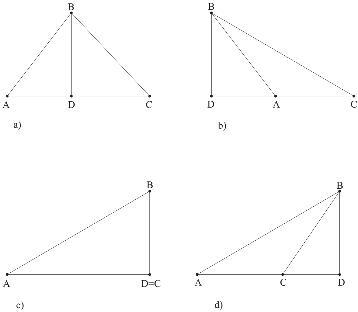
Figure 1.135: Illustration for proof of L 1.3.20.
