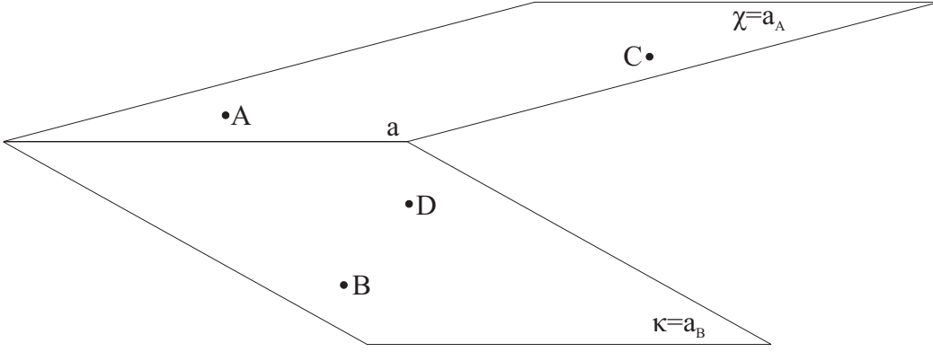
Figure 1.82: If points C, D lie, respectively, on the sides \chi = a_A, \kappa = a_B of the dihedral angle \widehat{\chi\kappa} then \widehat{CaD} = \widehat{\chi\kappa} .
