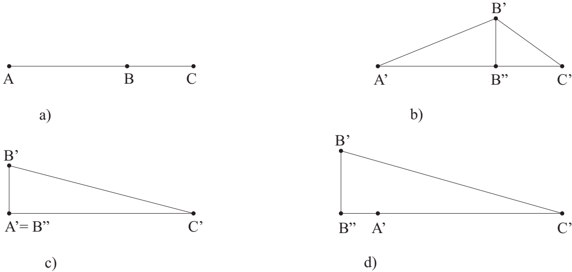
Figure 1.153: Illustration for proof of L 1.3.29.2.
