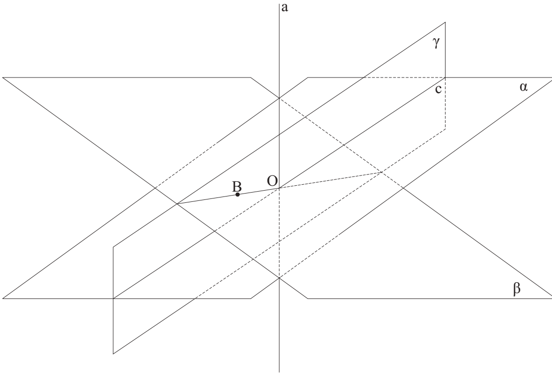
Figure 1.162: Illustration for proof of uniqueness in T 1.3.43.
