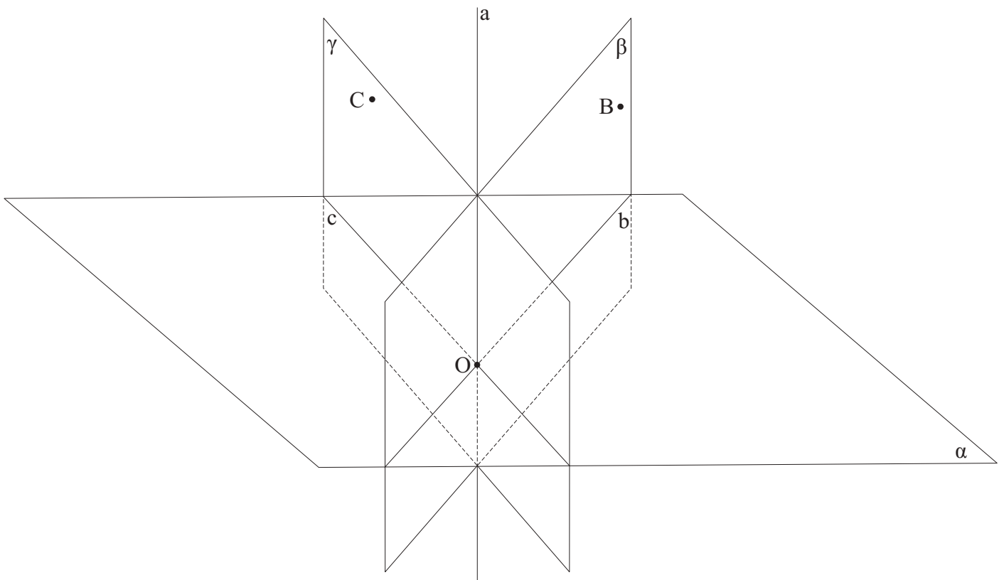
Figure 1.161: Illustration for proof of existence in T 1.3.43.
