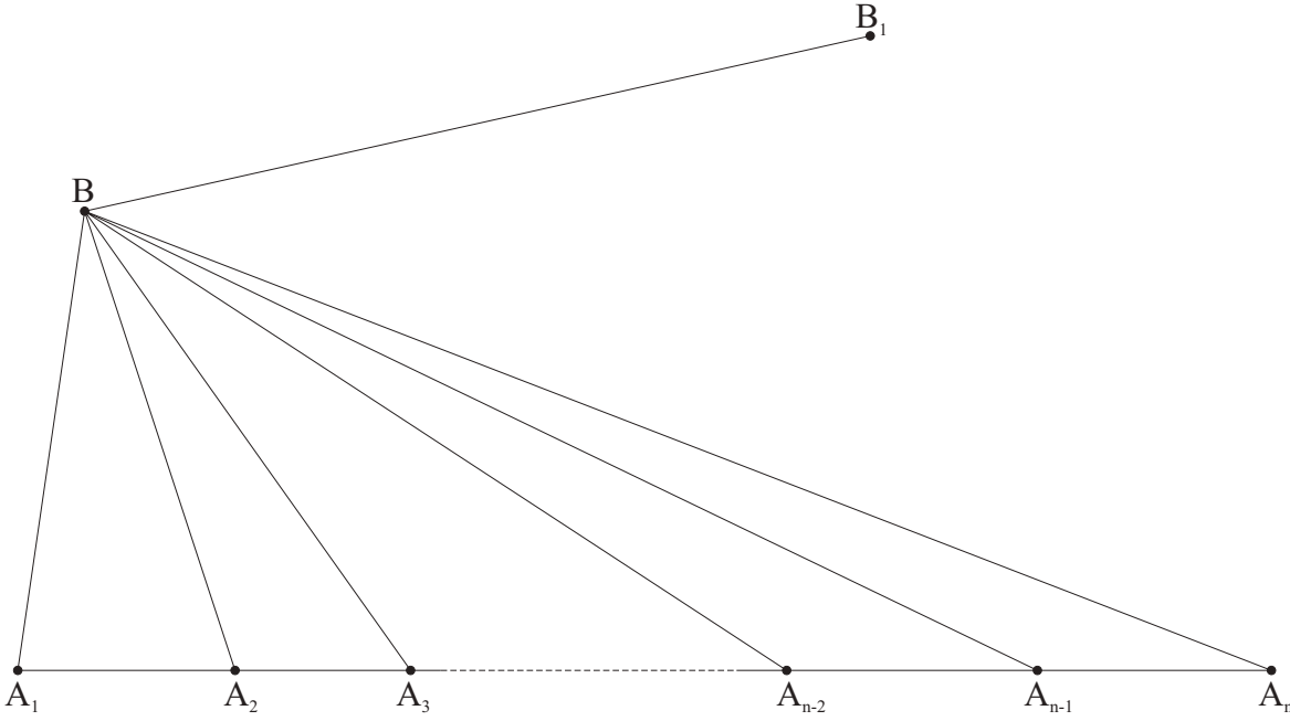
Figure 1.52: Suppose that a finite sequence of points A_i , where i \in \mathbb{N}_n , n \geq 3 , has the property that every point of the sequence, except for the first and the last, lies between the two points with adjacent (in \mathbb{N} ) numbers. Suppose, further, that a ray B_{B_1} does not meet the ray A_{1A_2} and that the points A_2, B_1 lie on the same side of the line a_{A_1B} . Then the rays B_{A_1}, B_{A_2}, \dots, B_{A_n} B_{B_1} are in order [B_{A_1} B_{A_2} \dots, B_{A_n} B_{B_1}] .
