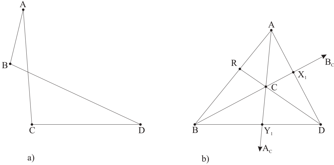
Figure 1.68: Illustration for proof of T 1.2.42.
