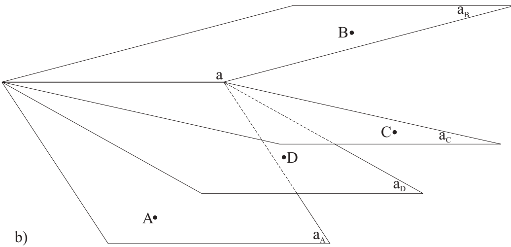
Figure 1.95: If a half-plane a_B lies inside a dihedral angle \widehat{AaC} , the ray a_C lies inside a dihedral \widehat{BaD} , and at least one of the half-planes a_B, a_C lies on the same side of the plane \alpha_{aA} as the half-plane a_D , then the half-planes a_B, a_C both lie inside the dihedral angle \widehat{AaD} .
