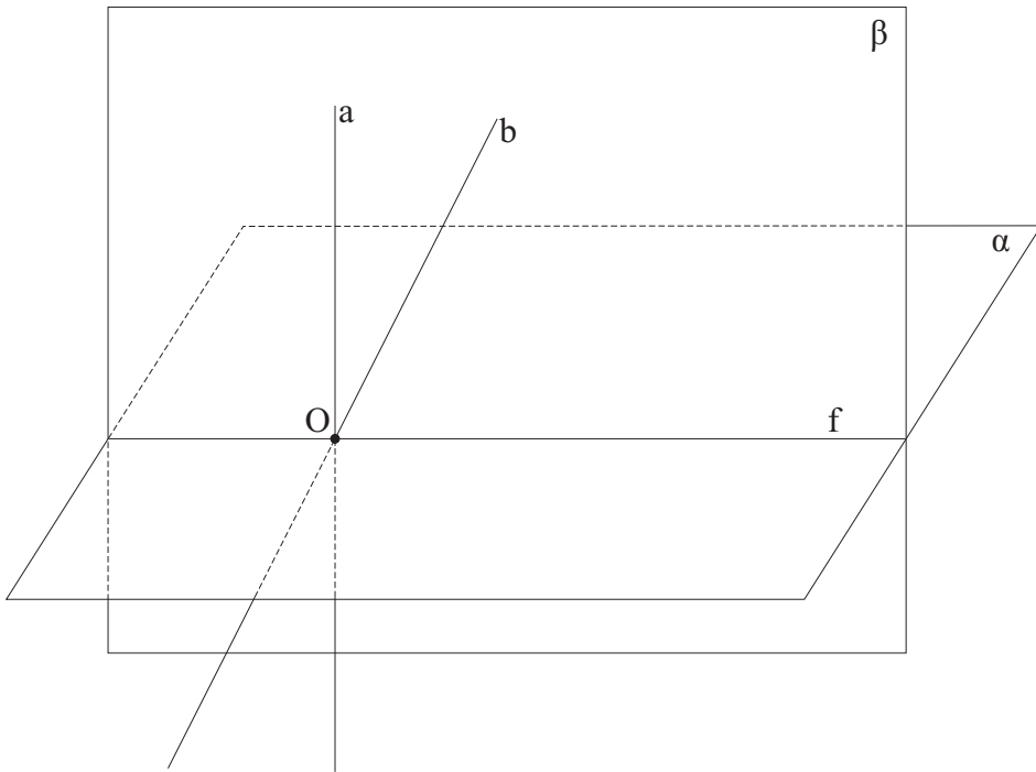
Figure 1.163: Illustration for proof of uniqueness in T 1.3.44.
