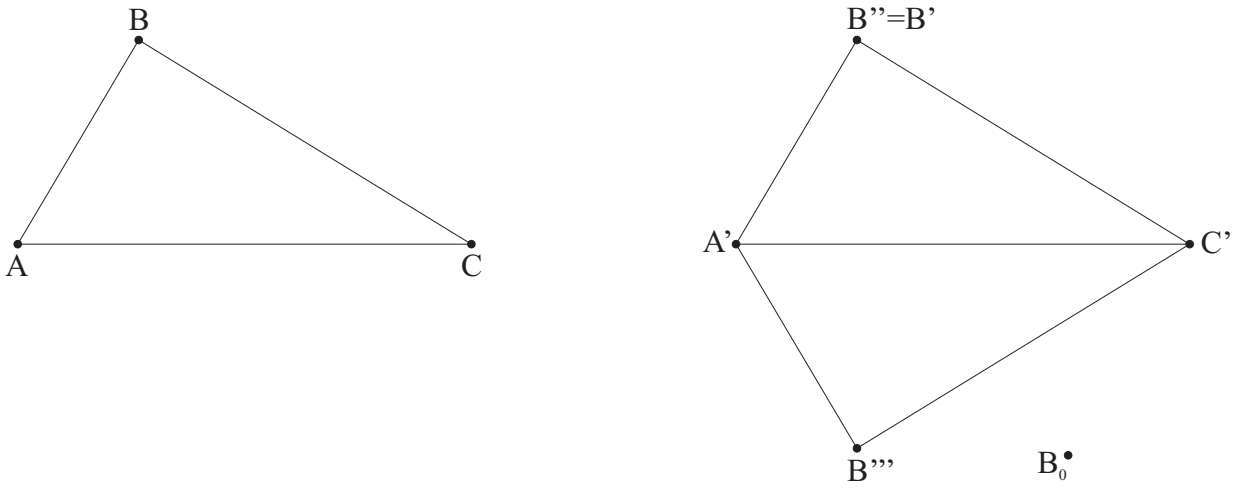
Figure 1.117: if AB \equiv A'B', BC \equiv B'C', AC \equiv A'C' , the triangle \triangle ABC is congruent to the triangle \triangle A'B'C' (SSS, or The Third Triangle Congruence Theorem ).
