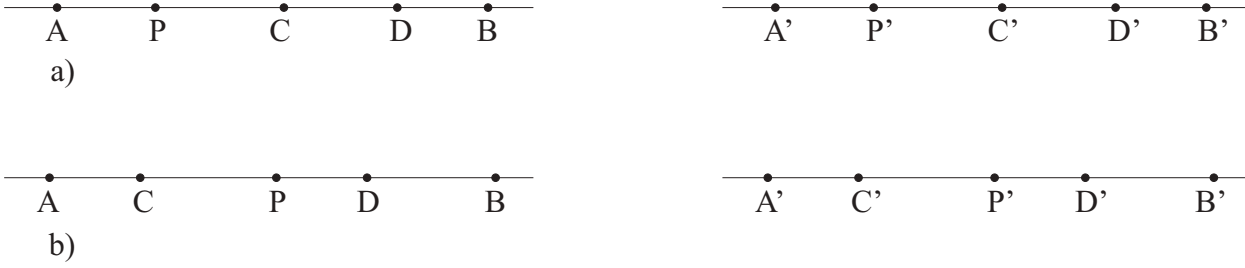
Figure 1.157: Illustration for proof of C 1.3.30.2.
