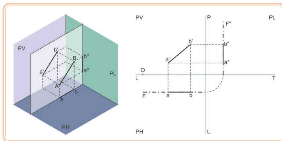
Figura 5.19: Plano frontal – reta frontal
