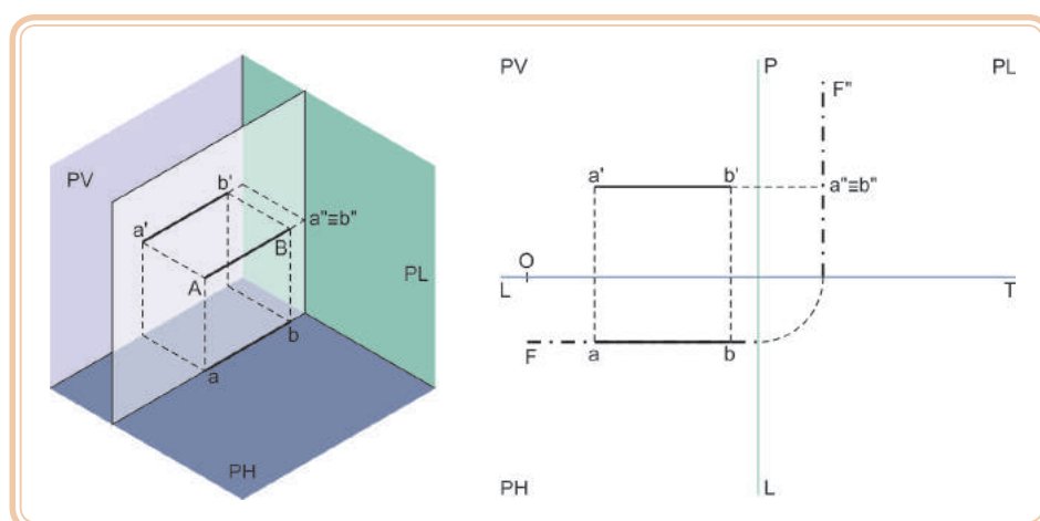
Figura 5.20: Plano frontal – reta fronto-horizontal
