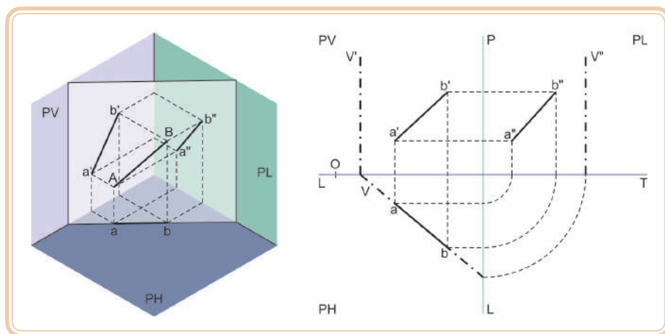
Figura 5.15: Plano vertical – reta oblíqua
