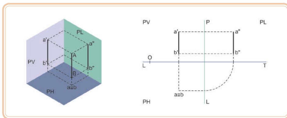
Figura 4.10: Reta vertical
