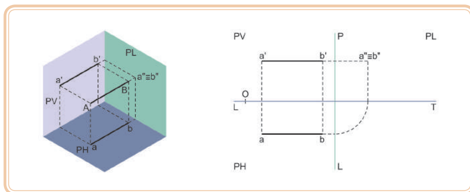
Figura 4.11: Reta fronto-horizontal
