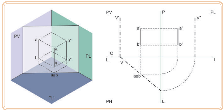
Figura 5.13: Plano vertical – reta vertical
