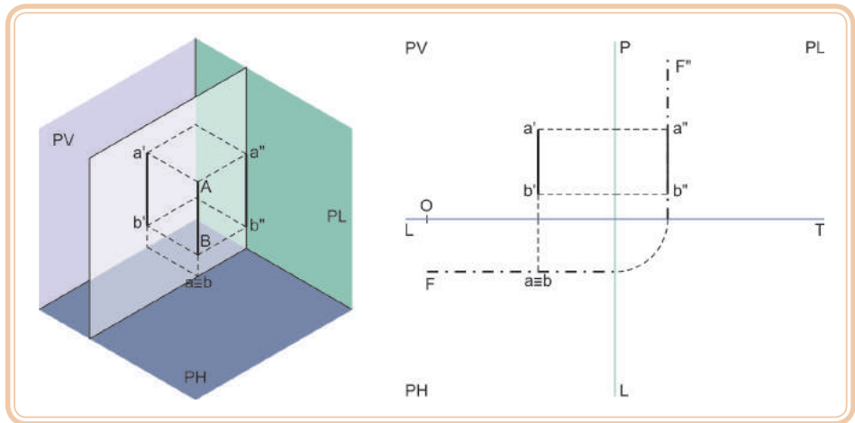
Figura 5.21: Plano frontal – reta vertical
