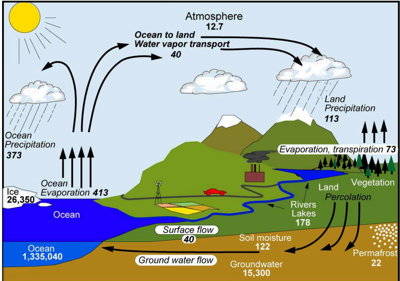
Figure 14: The Global Water Cycle. Fluxes are indicated in slanted font. From Trenberth et al. (2007). Image from ucar.edu .
