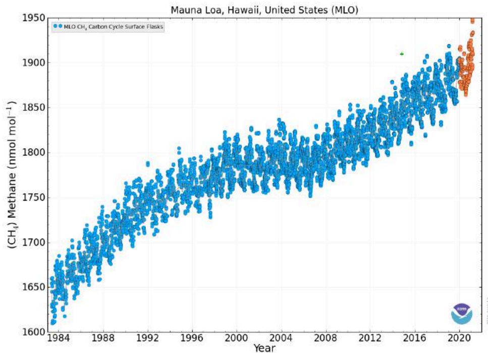
Figure 10: Top: Atmospheric methane concentrations as a function of time. Top: Recent air measurements from Mauna Loa. Bottom: Ice core, firn, and air measurements from Antarctica. Note that most methane sources are in the northern hemisphere, which leads to higher concentrations there compared with the southern hemisphere.
