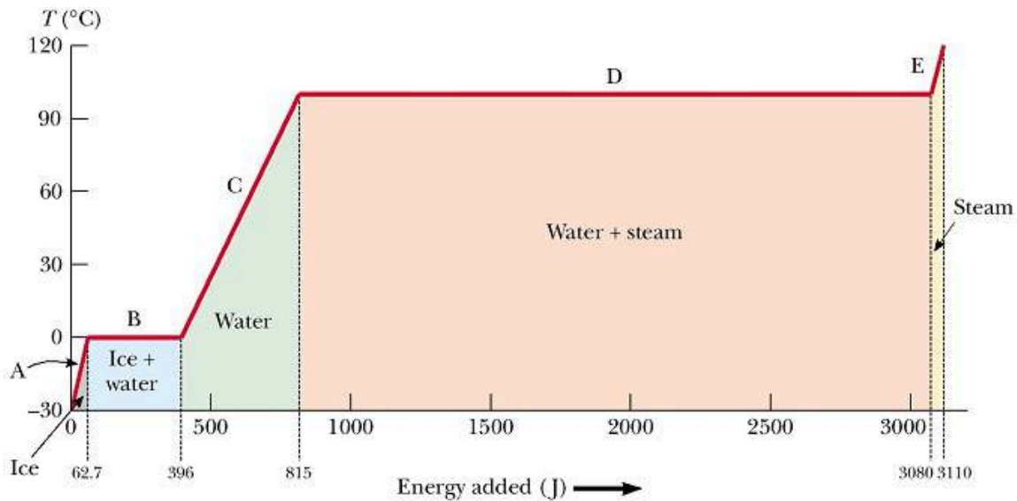
Figure 10: Effects of heat added ( \Delta H ) on the temperature of one gram of water. Starting from ice at -30^{\circ}\text{C} we need to add about 63 J to warm it up to the melting point (line A). About 333 J are required to melt the ice (line B). During this process the temperature stays constant. Once all ice is melted into water adding more heat causes the water temperature to increase until the boiling point (line C). The slope of line C is the heat capacity of water (at constant pressure) c_{p,\text{water}} = \Delta H/\Delta T = 4.2 \text{ J}/(\text{g}^{\circ}\text{C}) . Once the water boils any added heat is used to vaporize water and the temperature stays at the boiling point until all water is vaporized. The latent heat of vaporization is \sim 2270 \text{ J}/\text{g} . Thus, the energy required to vaporize water is more than five times as much as to warm it from 0^{\circ}\text{C} to 100^{\circ}\text{C} .
