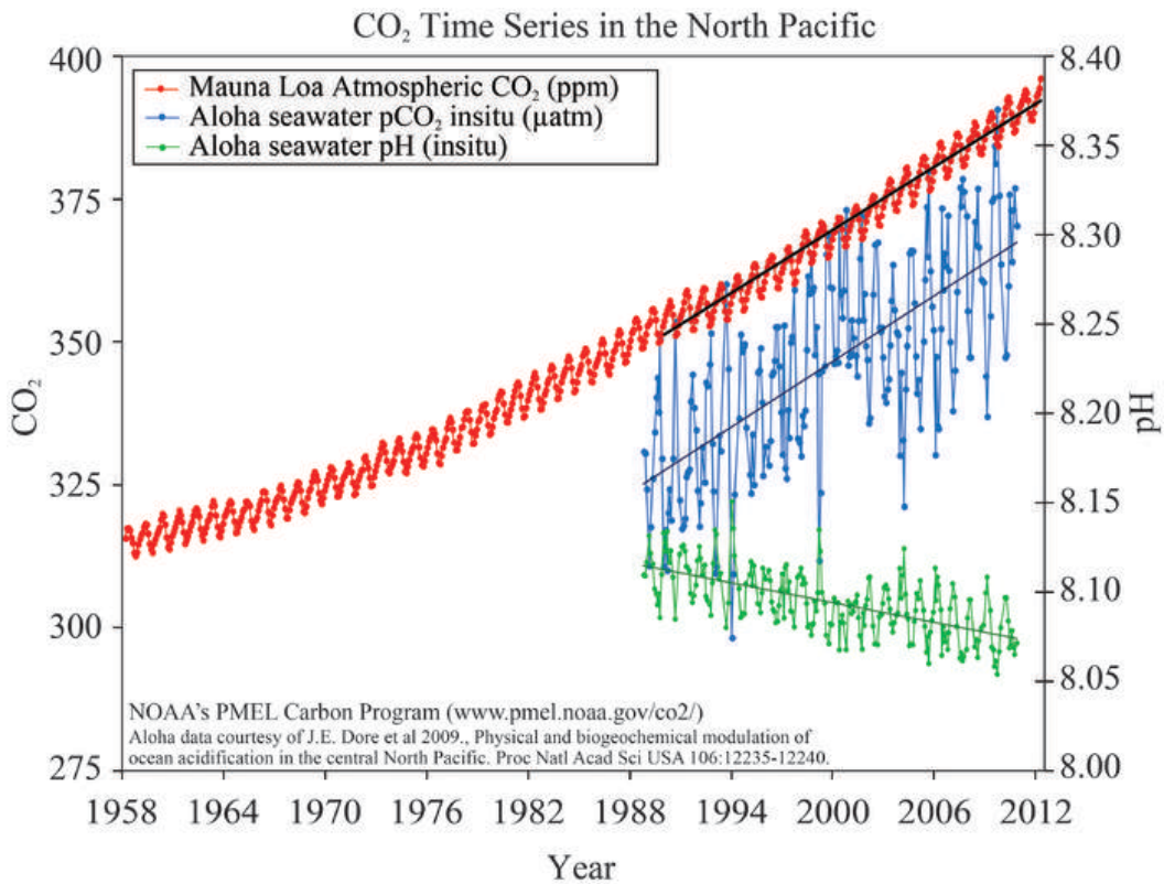
Figure 11: Measurements of seawater p\text{CO}_2 (blue) and pH (green) at ocean station Aloha near Hawaii together with the Mauna Loa record of atmospheric \text{CO}_2 (red). From pmel.noaa.gov .
