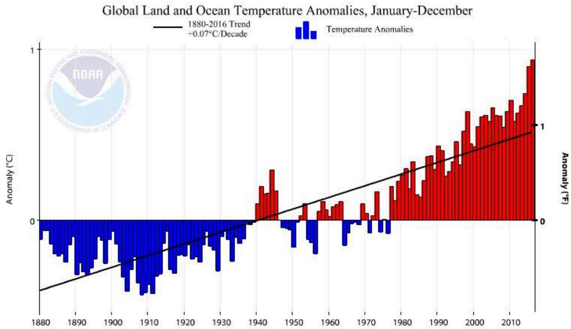
Figure 12: Averaged over land and ocean the increase in Earth's temperature over the past 100 years has been approximately 0.7^{\circ}\text{C} ( 0.07^{\circ}\text{C}/\text{decade} ). This result is very robust. Several groups around the world have analyzed the available data in different ways and came to the same conclusion. This is a key figure.
