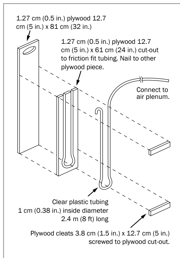
Figure 12–1. Home-built manometer.
