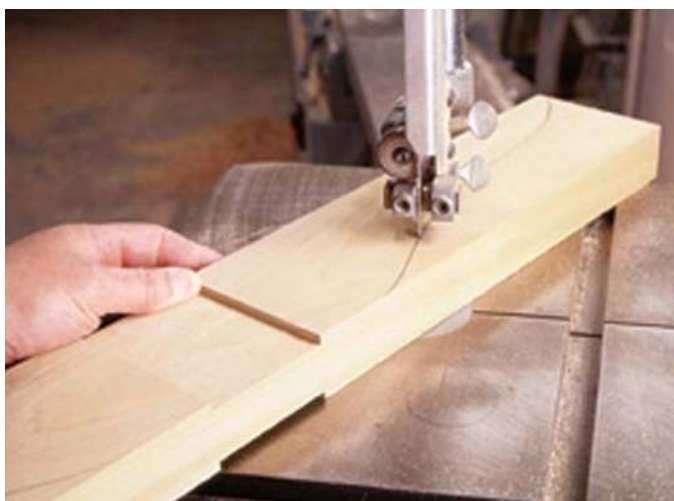
Sculpting a shape on the cross braces isn't necessary to keep the table sturdy, but it does keep it from looking clunky. After transferring the pattern onto the brace, I cut wide of the line on the band saw, then used a spindle sander to smooth the shape.
