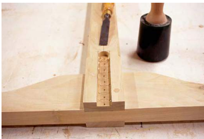
Here's the mortise for the stretcher. I removed most of the waste with a Forstner bit, then chiseled the mortise square.
