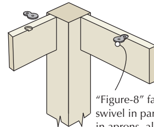
"Buttons" will slide in slots in aprons, allowing top to move.
