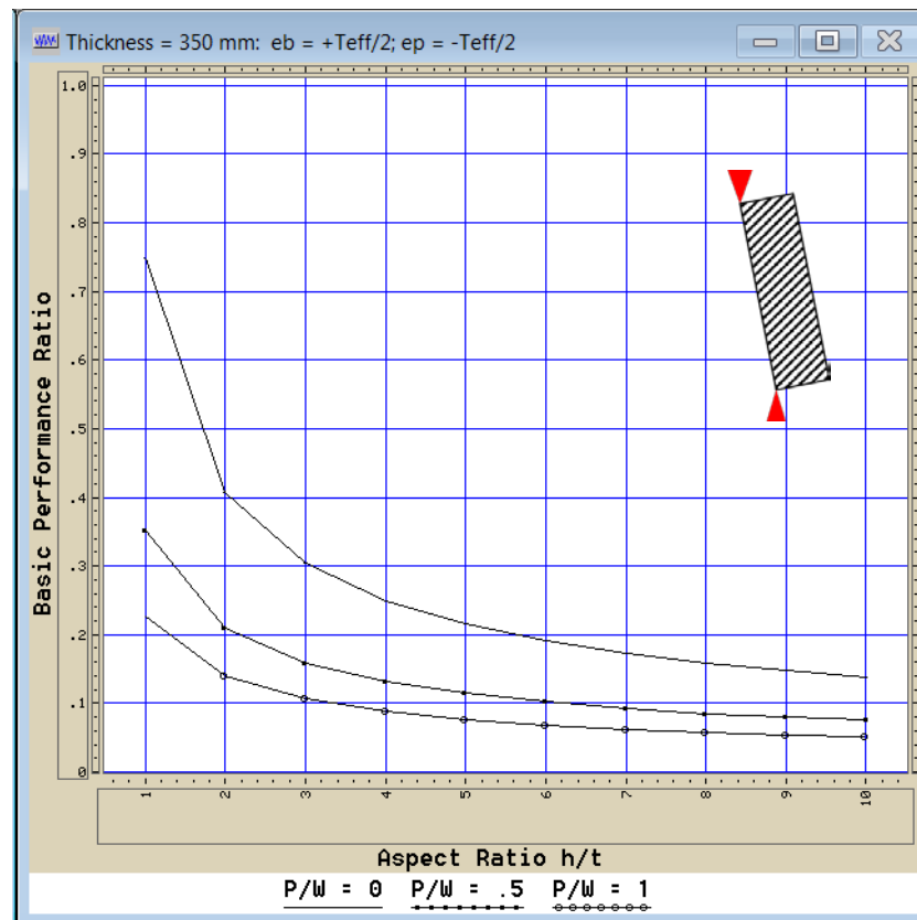
Figure C8C.9: 350 mm thick cantilever wall
