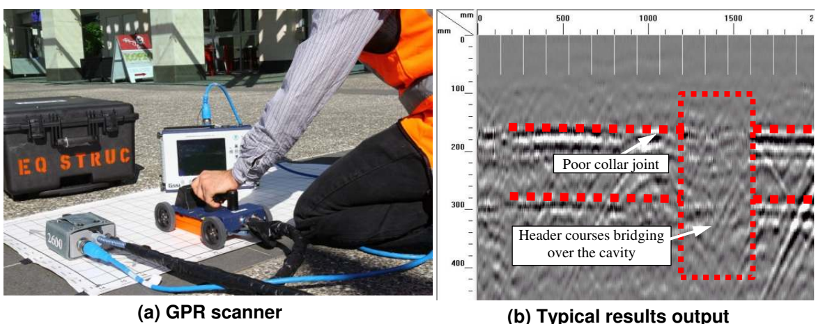
Figure C8A.9: Example of non-invasive scanning using Ground Penetrating Radar (GPR) scanner technology (EQ STRUC Ltd)
