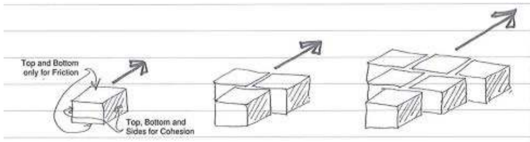
Figure C8.61: Basis for embedded anchor capacity estimation
