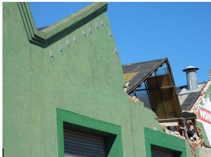
Figure C8.40: Collapse of gable wall. Note a secured gable end that survived earthquake loading and a companion failed gable end that was not secured. (Ingham and Griffith, 2011)
