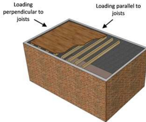
Figure C8.59: Orthogonal diaphragm response due to joist orientation
