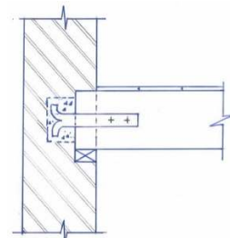
(d) Fish-tail connection between wall and joist
