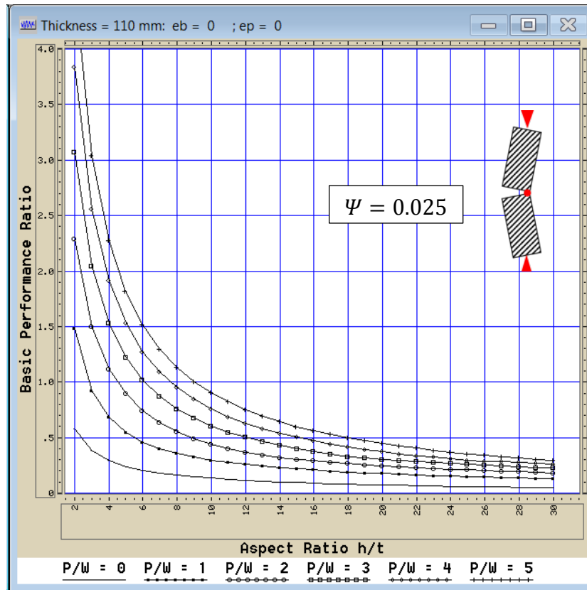
(e) For e_b = 0 and e_p = 0 ( t_{\text{Gross}} = 110 mm)
