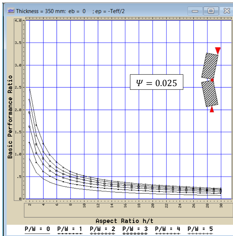
f) For e_b = 0 and e_p = -t/2 ( t_{\text{Gross}} = 350 mm)
