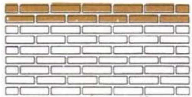
(b) Running bond
