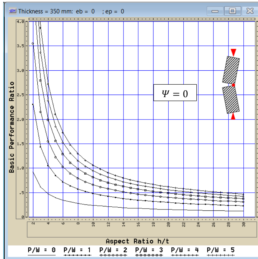
(e) For e_b = 0 and e_p = 0 ( t_{\text{Gross}} = 350 mm)
