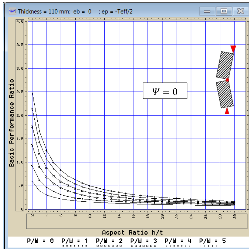
(f) For e_b = 0 and e_p = -t/2 ( t_{\text{Gross}} = 110 mm)
