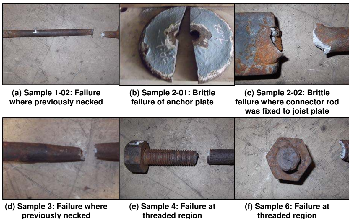
Figure C8.36: Observed failure modes from tensile test series (Campbell et al., 2012)
