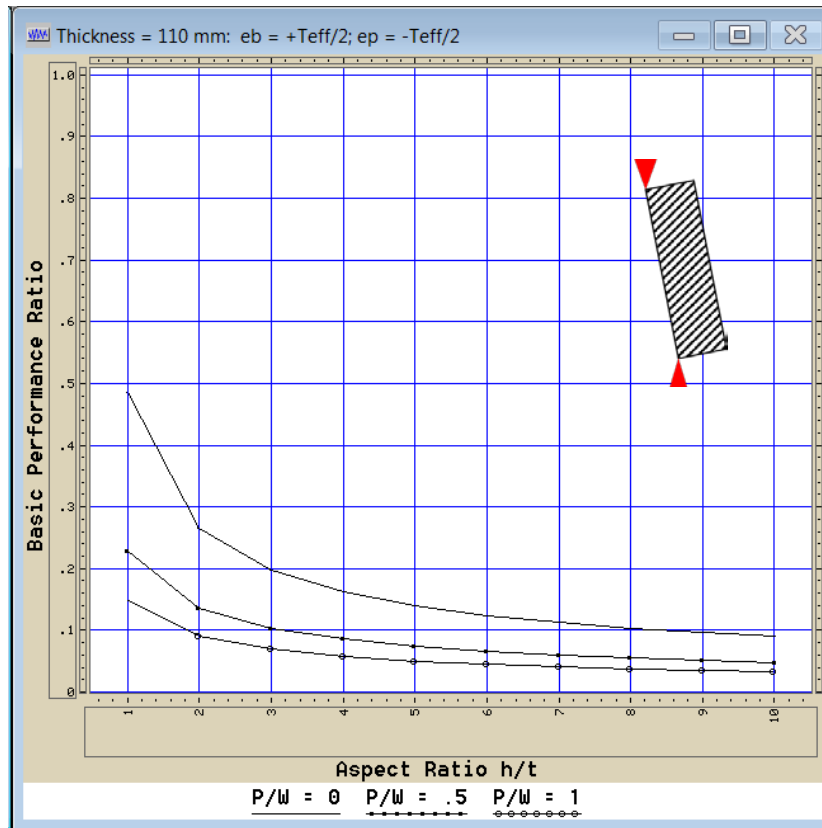
Figure C8C.7: 110 mm thick cantilever wall
