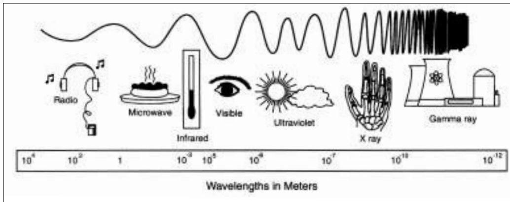
Figure 1: Electromagnetic Spectrum
