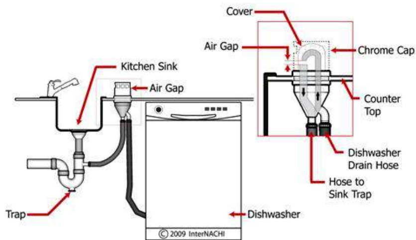
Dishwasher Air Gap
