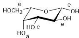
\beta -D-Galactopyranose
