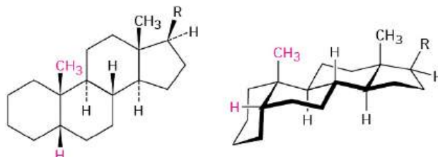
FIGURE 27.12 Steroid conformations. The three 6-membered rings have chair conformations but are unable to undergo ring-flips. The A and B rings can be either cis-fused or trans-fused.
