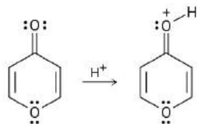
4-Pyrone
