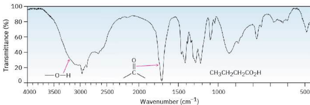
FIGURE 20.6 IR spectrum of butanoic acid, CH_3CH_2CH_2CO_2H .
