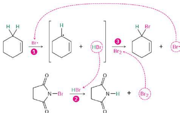
FIGURE 10.3 Mechanism of allylic bromination of an alkene with NBS. The process is a radical chain reaction in which (1) a Br• radical abstracts an allylic hydrogen atom of the alkene and gives an allylic radical plus HBr. (2) The HBr then reacts with NBS to form Br 2 , which (3) reacts with the allylic radical to yield the bromoalkene product and a Br• radical that continues the chain.
