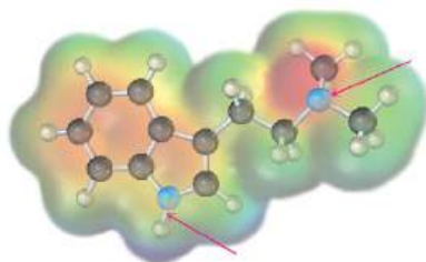
N,N -Dimethyltryptamine
