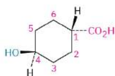
trans-4-Hydroxycyclohexanecarboxylic acid
