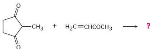
2-Methyl-1,3-cyclo- pentanedione
