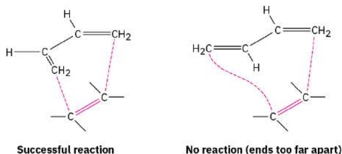
Successful reaction
