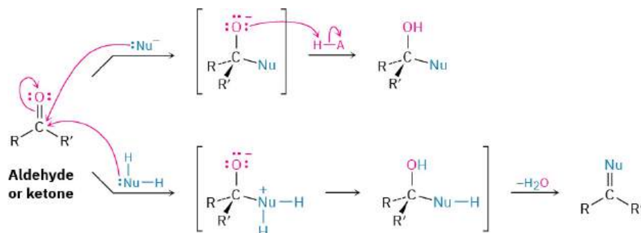
FIGURE 18.9 The addition reaction of an aldehyde or a ketone with a nucleophile. Depending on the nucleophile, either an alcohol or a compound with a \text{C=Nu} double bond is formed.
