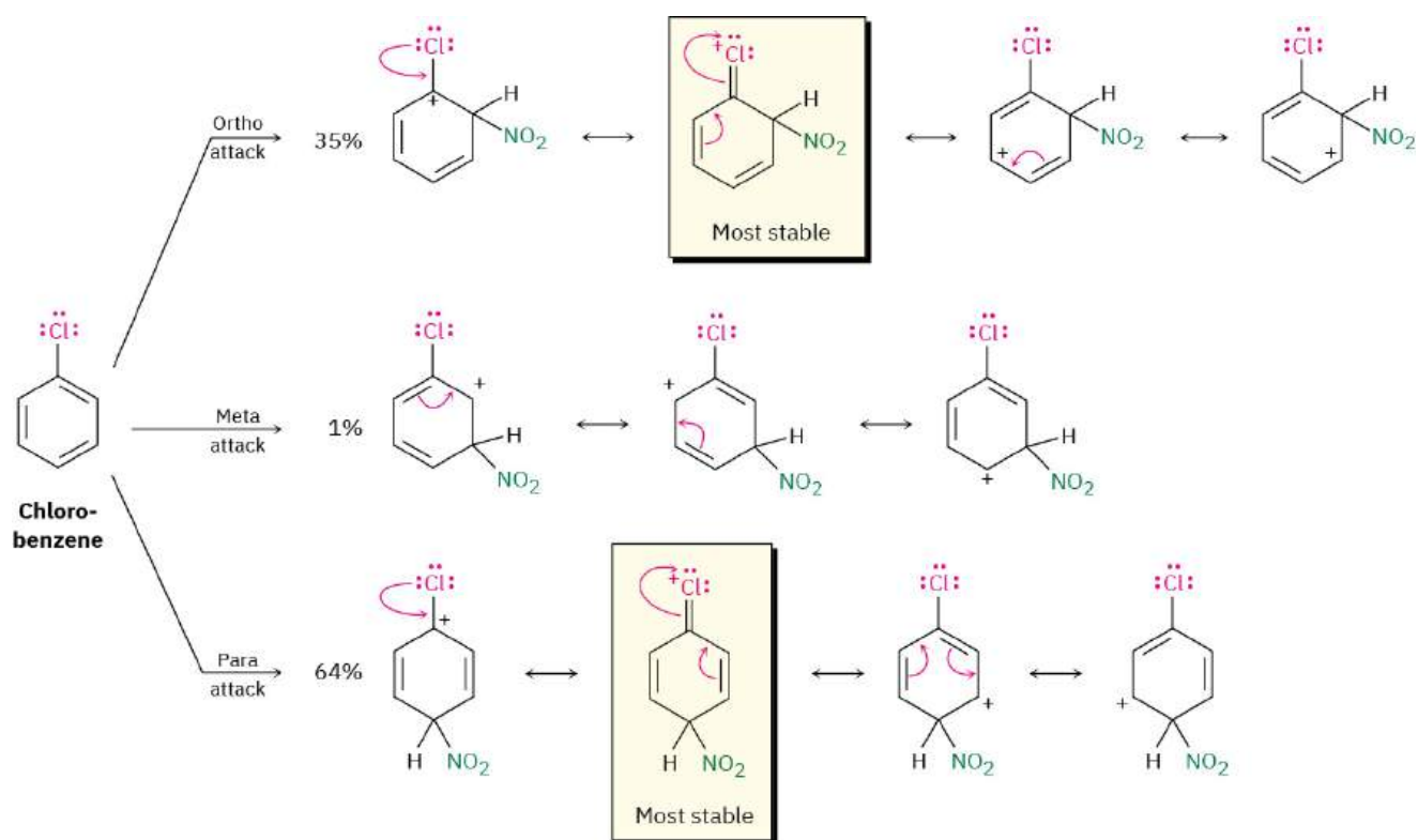
FIGURE 16.16 Carbocation intermediates in the nitration of chlorobenzene. The ortho and para intermediates are more stable than the meta intermediate because of electron donation of the halogen lone-pair electrons.
