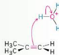
2-Methylpropene
