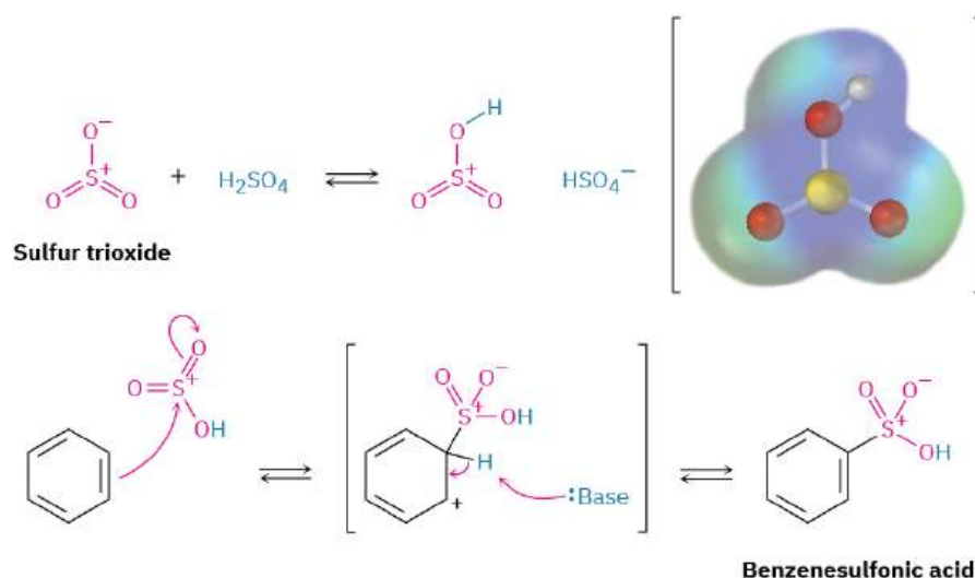
FIGURE 16.6 The mechanism for electrophilic sulfonation of an aromatic ring. An electrostatic potential map of the reactive electrophile \text{HOSO}_2^+ shows that sulfur and hydrogen are the most positive atoms .
