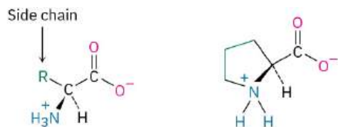
A primary α-amino acid
