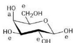
\beta -D-Galactopyranose
