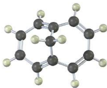
1,6-Methanonaphthalene
