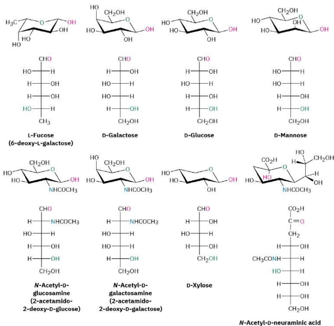
FIGURE 25.10 Structures of the eight monosaccharides essential to humans.
