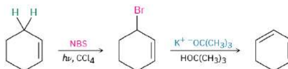
Cyclohexene 3-Bromocyclohexene 1,3-Cyclohexadiene (76%)
