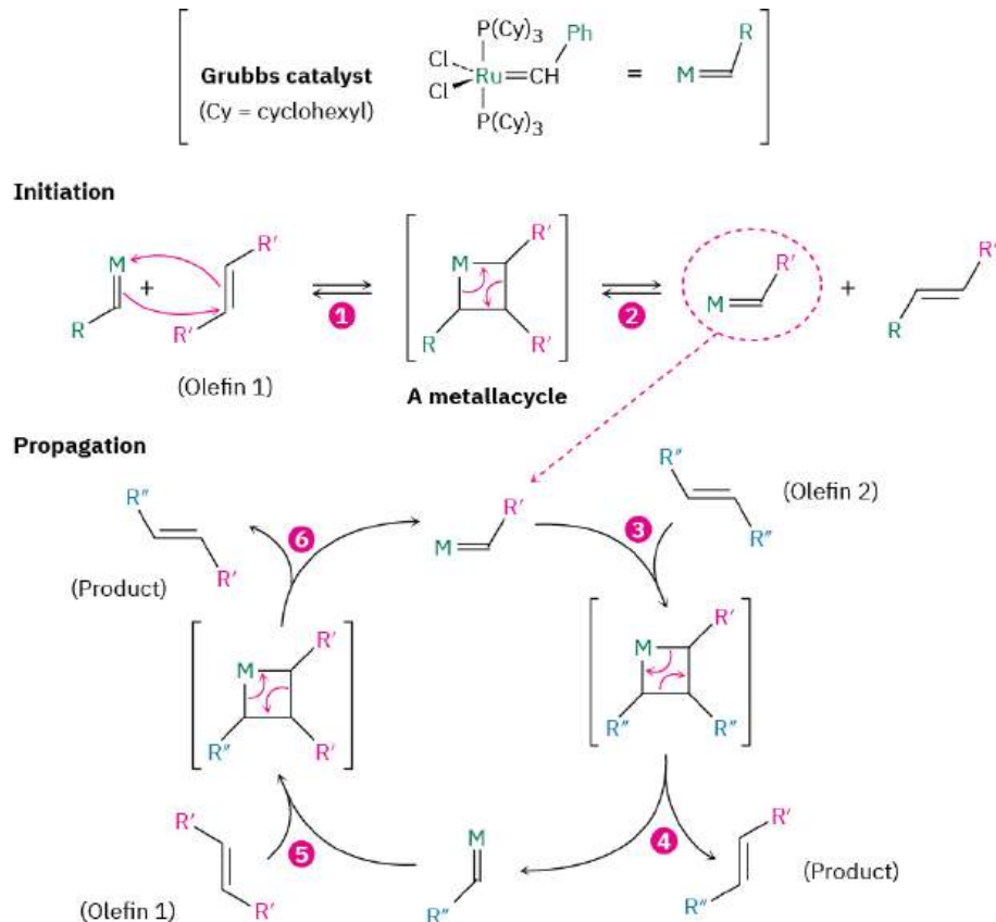
FIGURE 31.3 Mechanism of the olefin metathesis reaction. The process is initiated by a two-step sequence that involves (1) reaction of the catalyst and olefin 1 to give a four-membered metallacycle intermediate, followed by (2) ring-opening to give a different form of catalyst that contains part of olefin 1. (3) Reaction of this new catalyst with olefin 2 gives another metallacycle intermediate, (4) which opens to give metathesis product and another form of catalyst. (5, 6) The repeating ring-forming and ring-opening steps then continue.
