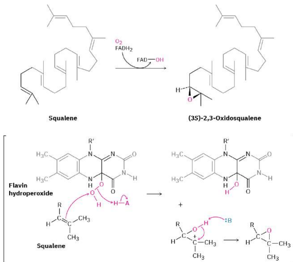
FIGURE 27.14 Proposed mechanism of the oxidation of squalene by flavin hydroperoxide.
