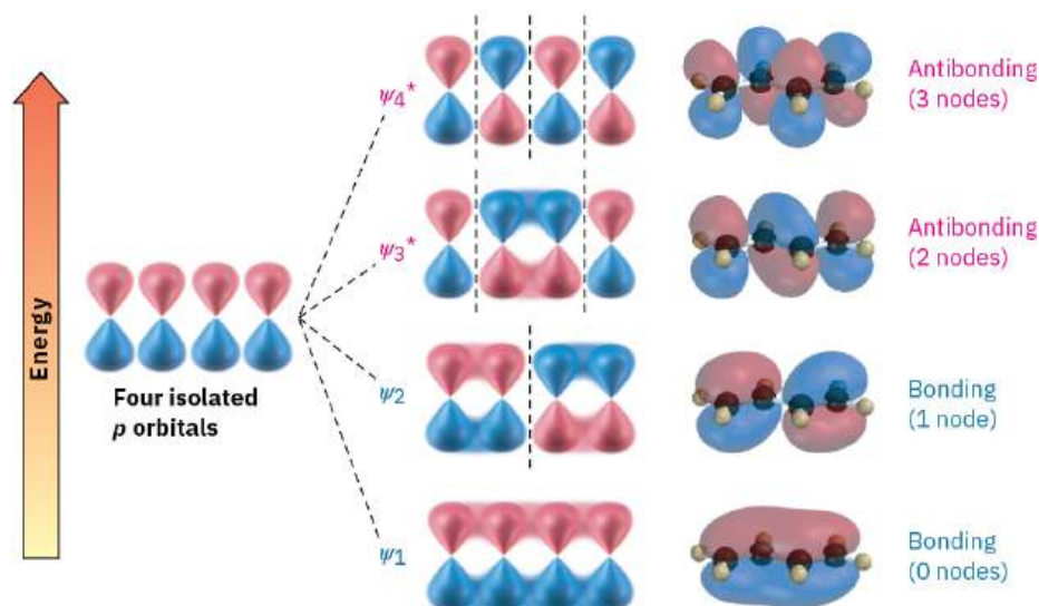
FIGURE 14.3 Four \pi molecular orbitals in 1,3-butadiene. Note that the number of nodes between nuclei increases as the energy level of the orbital increases.
