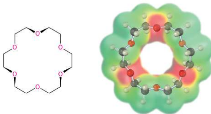
18-Crown-6 ether
