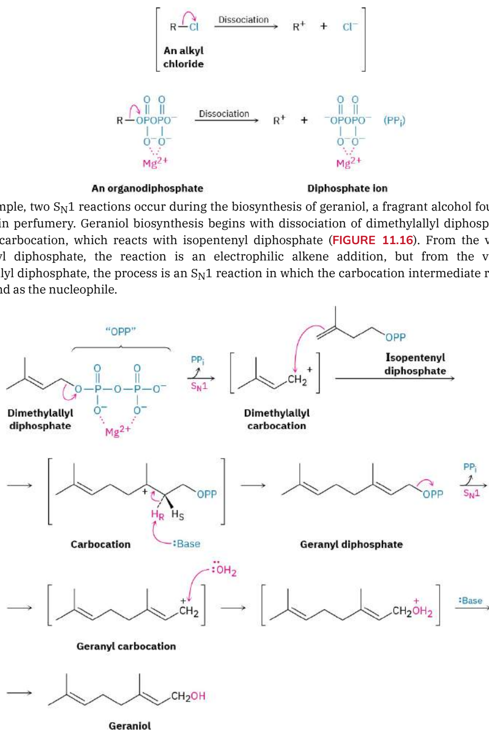
FIGURE 11.16 Biosynthesis of geraniol from dimethylallyl diphosphate. Two S_N1 reactions occur, both with diphosphate ion as the leaving group.
