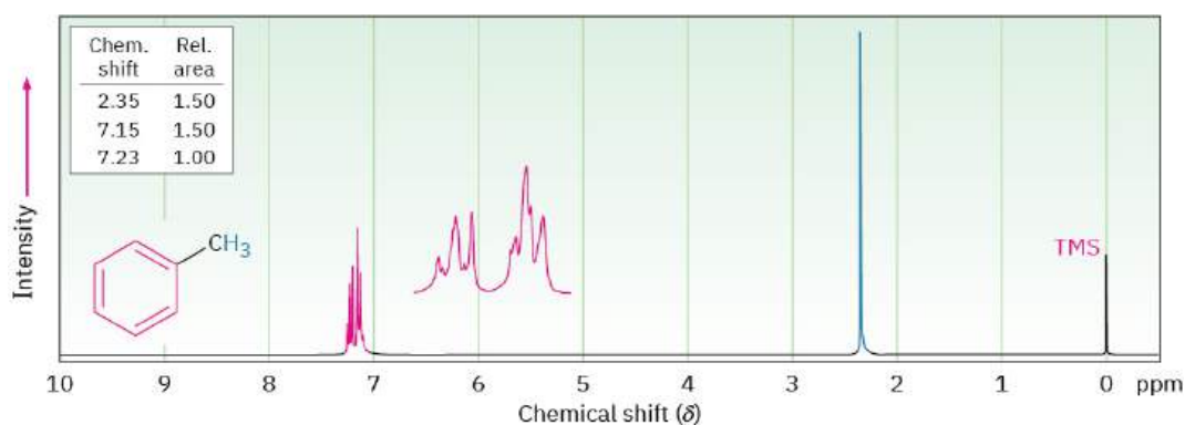
FIGURE 13.13 The ^1\text{H} NMR spectrum of toluene, showing the accidental overlap of the five nonequivalent aromatic ring protons.
