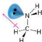
Methylamine ( \mu = 1.31 )
