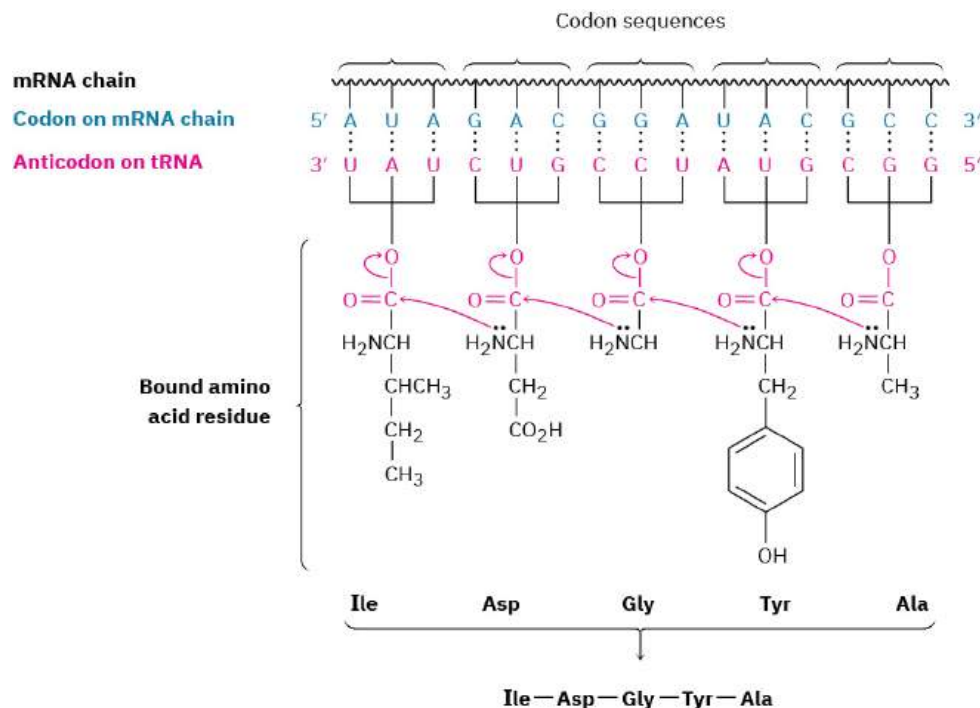
FIGURE 28.8 A representation of protein biosynthesis. The codon base sequences on mRNA are read by tRNAs containing complementary anticodon base sequences. Transfer RNAs assemble the proper amino acids into position for incorporation into the growing peptide.
