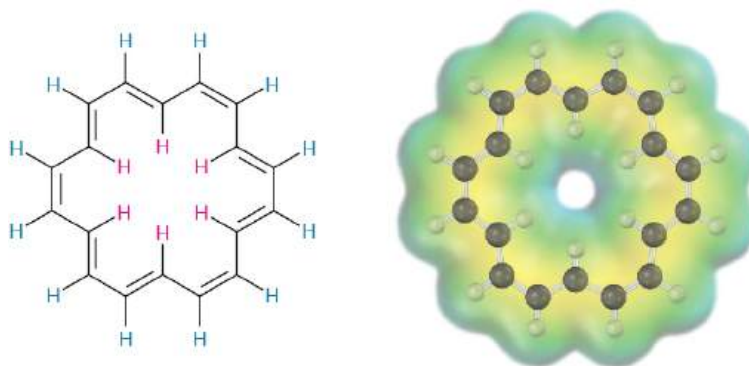
[18]Annulene
