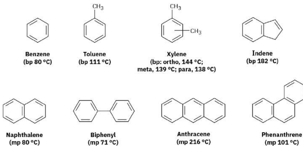
FIGURE 15.2 Some aromatic hydrocarbons found in coal tar.
