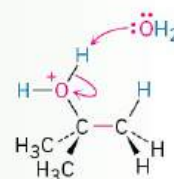
Protonated alcohol
