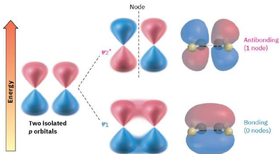
FIGURE 14.2 Two p orbitals combine to form two \pi molecular orbitals. Both electrons occupy the low-energy, bonding orbital, leading to a net lowering of energy and formation of a stable bond. The asterisk on \psi_2^* indicates an antibonding orbital.
