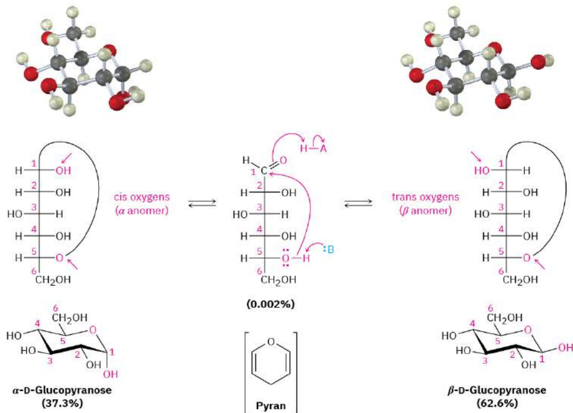
FIGURE 25.5 Glucose in its cyclic pyranose forms. As explained in the text, two anomers are formed by cyclization of glucose. The molecule whose newly formed \text{-OH} group at C1 is cis to the oxygen atom on the lowest chirality center (C5) in a Fischer projection is the \alpha anomer. The molecule whose newly formed \text{-OH} group is trans to the oxygen atom on the lowest chirality center in a Fischer projection is the \beta anomer.
