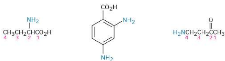
2-Aminobutanoic acid
