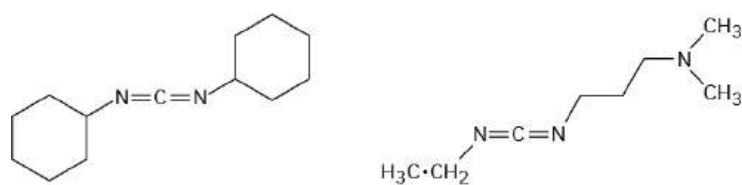
Dicyclohexylcarbodiimide 1-Ethyl-3-(3-dimethylaminopropyl)-carbodiimide
