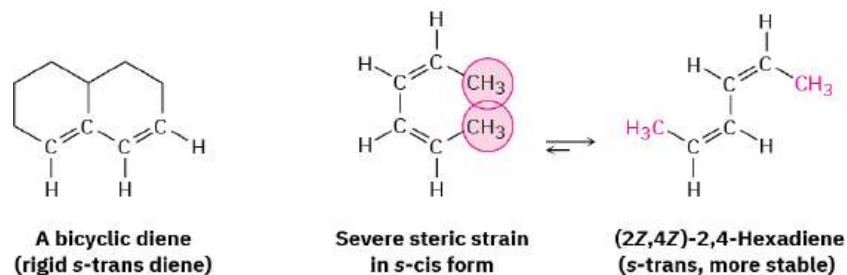
FIGURE 14.10 Two dienes that can't achieve an s-cis conformation and thus can't undergo Diels–Alder reactions.
