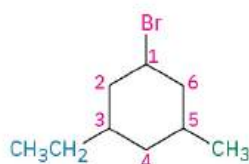
1-Bromo-3-ethyl-5-methylcyclohexane
