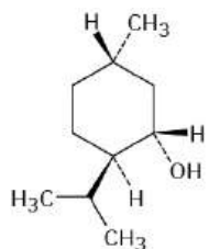
Menthol (from peppermint oil)
