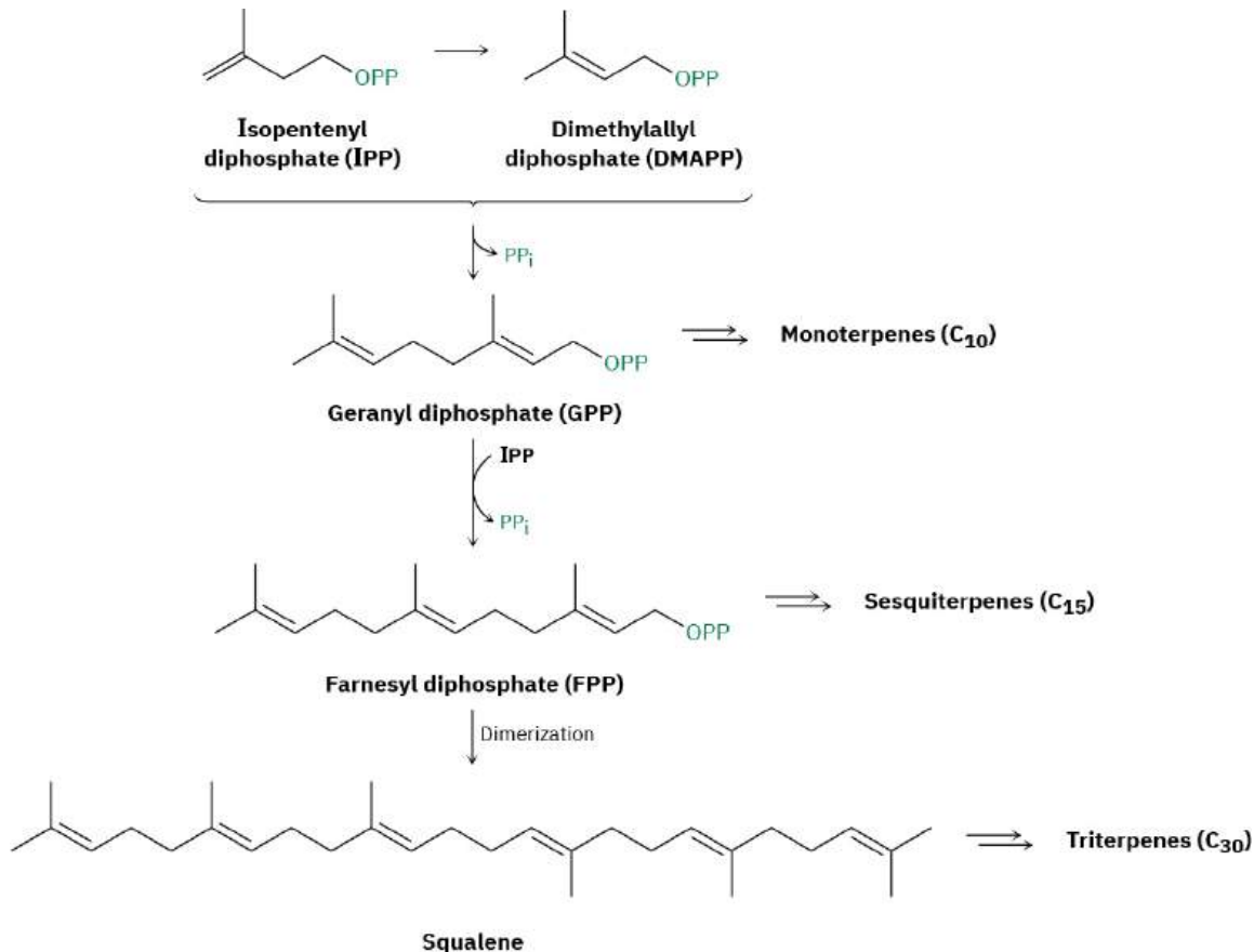
FIGURE 27.9 An overview of terpenoid biosynthesis from isopentenyl diphosphate.
