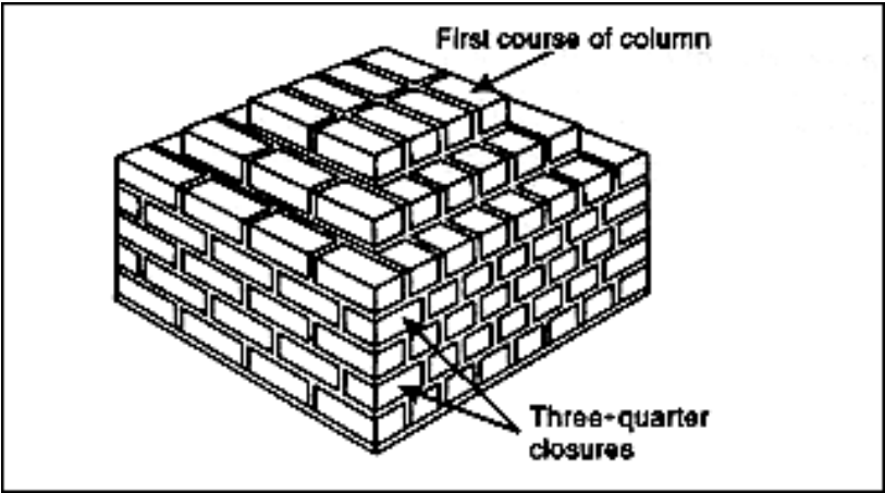
Figure 9-20. Column footing
