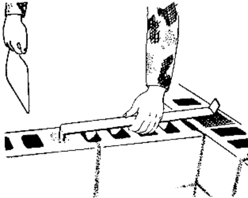
View 1. Z-shaped tie bar has right angle bends at each end
