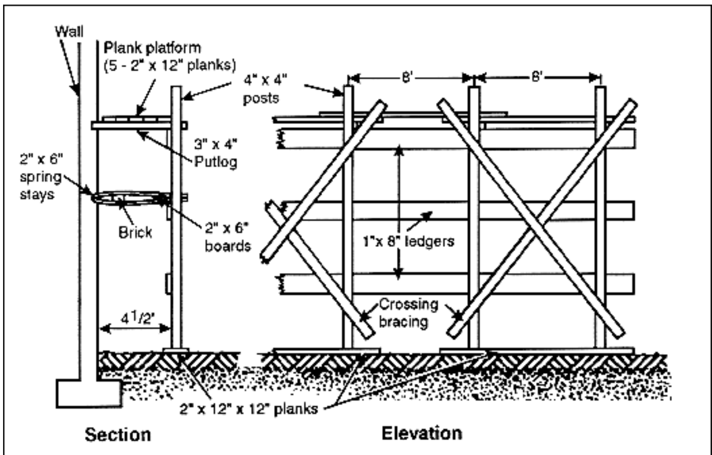
Figure 7-6. Putlog scaffold
