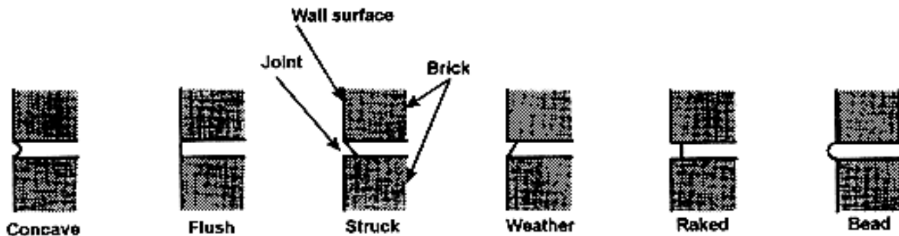
Figure 9-18. Joint finishes
