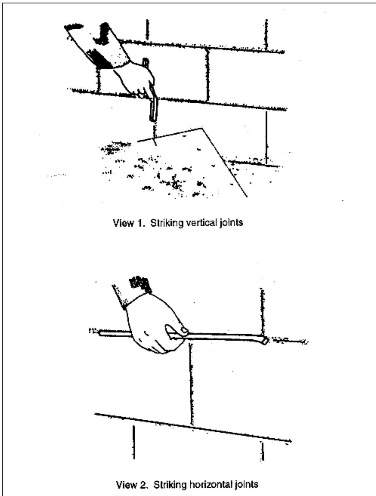
Figure 8-15. Tooling mortar joints
