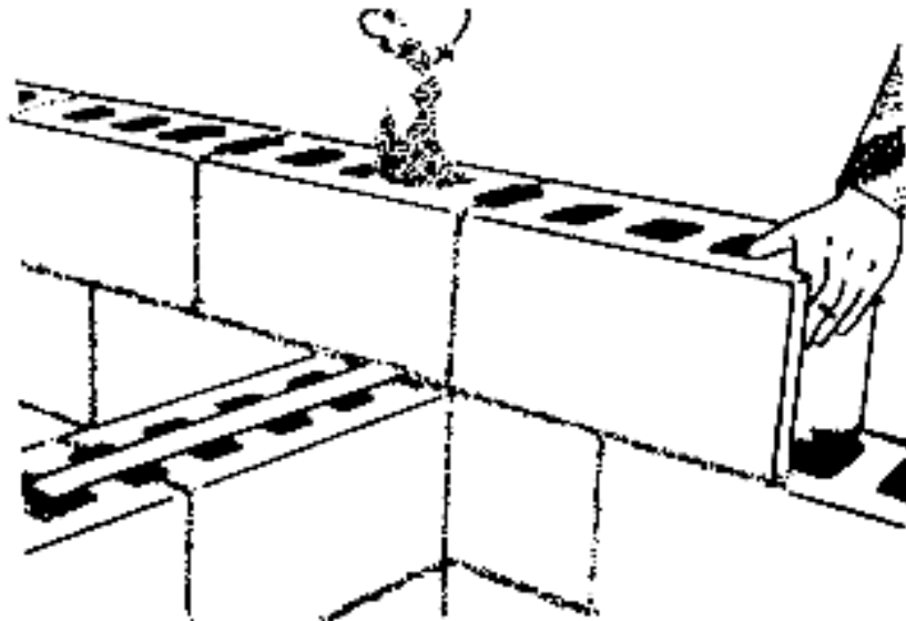
View 2. Filling core with mortar or concrete
