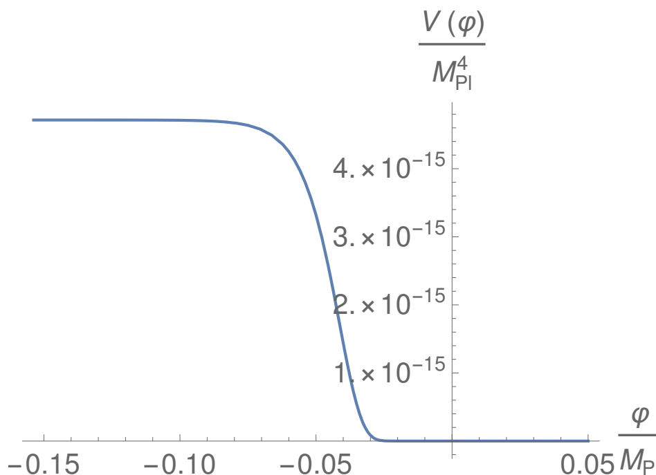
Figure 1. The \alpha -attractor potential. In Lorentzian QI, the corresponding potential has a similar shape.
