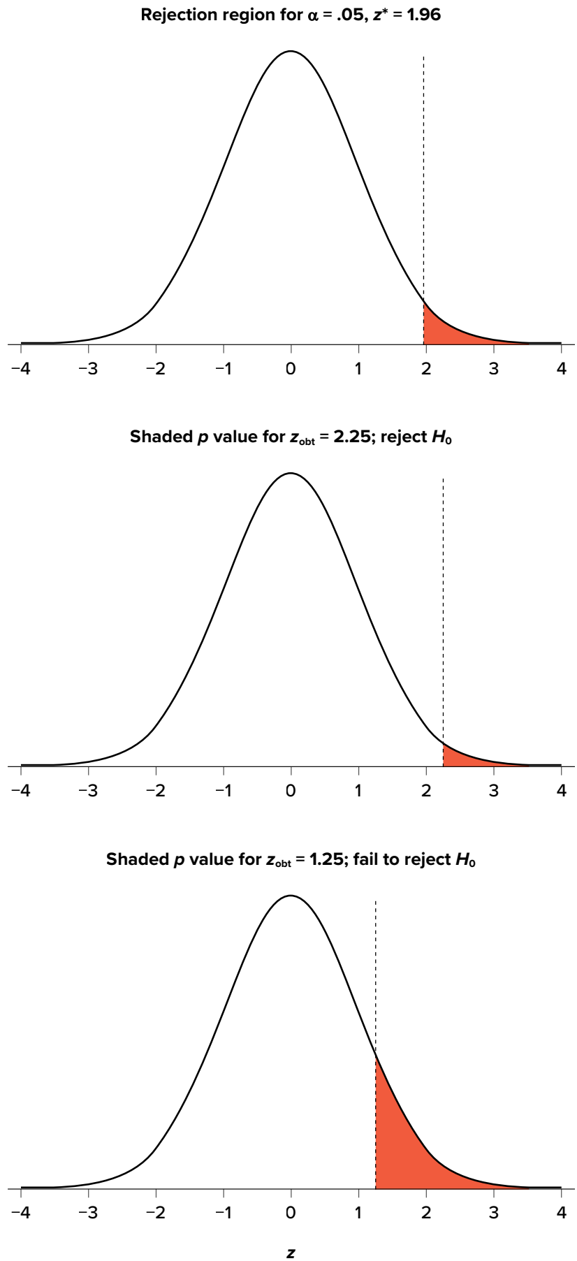
FIGURE 7.3. Relationship between \alpha , z_{\text{obt}} , and p . (“ Relationship between alpha, z-obt, and p ” by Judy Schmitt is licensed under CC BY-NC-SA 4.0 .)
