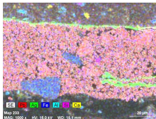
Figure 7. Cross-section viewed at 1000x (EDS mapping): Sample from blue colour on the cloak of the Virgin.
