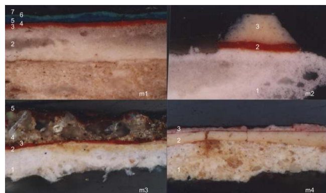
Figure 6. Optical microscopy. Photograph of cross sections of the samples analysed. © Enriqueta González Martínez.
