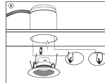
6" Can/J-box and Ceiling
