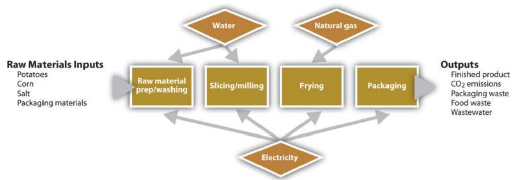
Figure 5.11 Production Process at Casa Grande, Arizona, Plant
