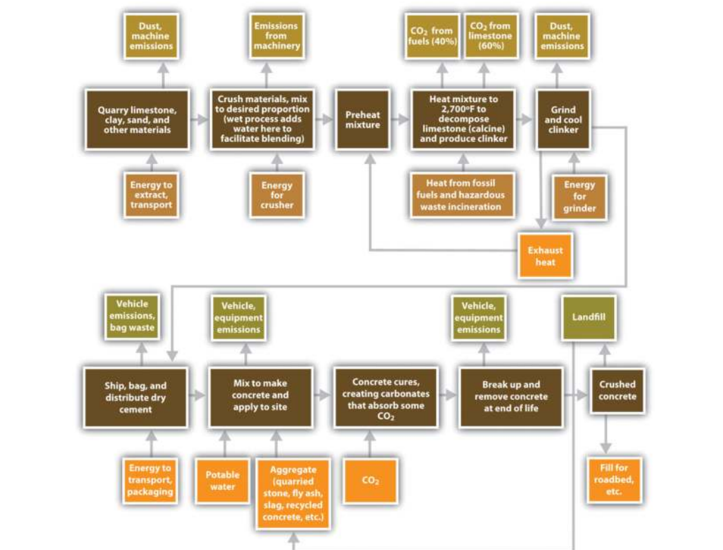
Figure 5.15 Life Cycle for Portland Cement Produced by Dry Process and Mixed into Concrete
