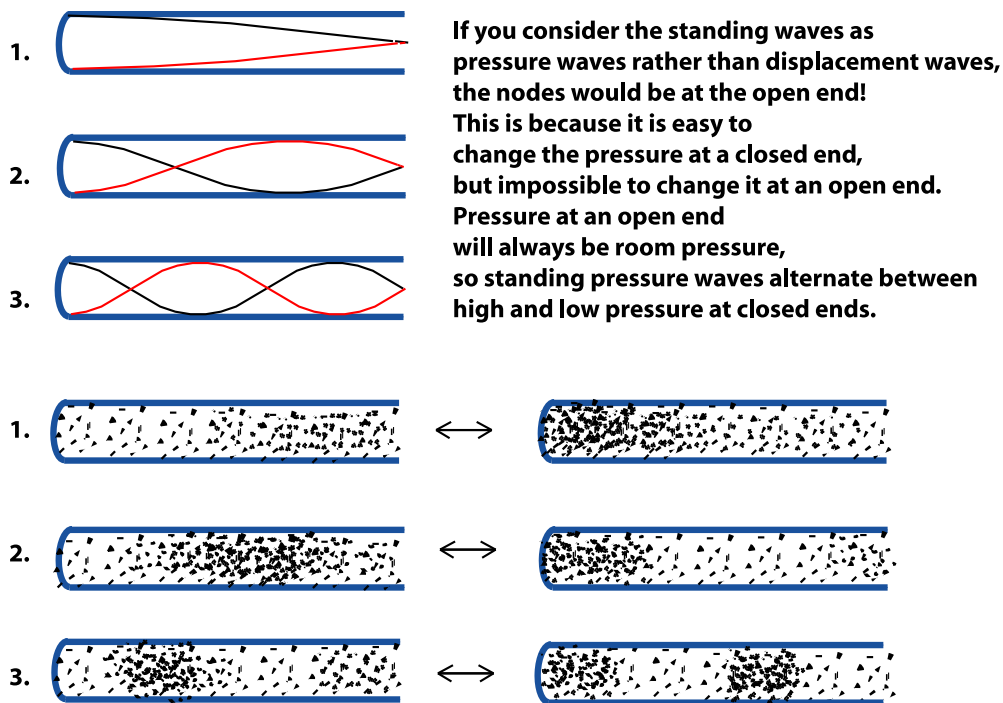
Figure 3.11: The standing waves in the tubes are actually longitudinal sound waves. Here the displacement standing waves in Figure 3.10 are shown instead as longitudinal air pressure waves. Each wave would be oscillating back and forth between the state on the right and the one on the left. See Standing Waves in Wind Instruments 19 for more explanation.
