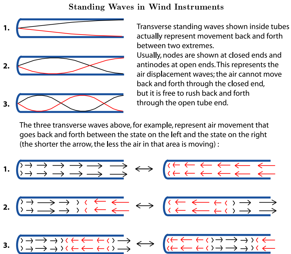
Figure 3.10: Standing Waves in a wind instrument are usually shown as displacement waves, with nodes at closed ends where the air cannot move back-and-forth.
