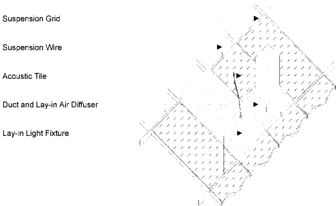
Fig. 2 Suspended ceiling
