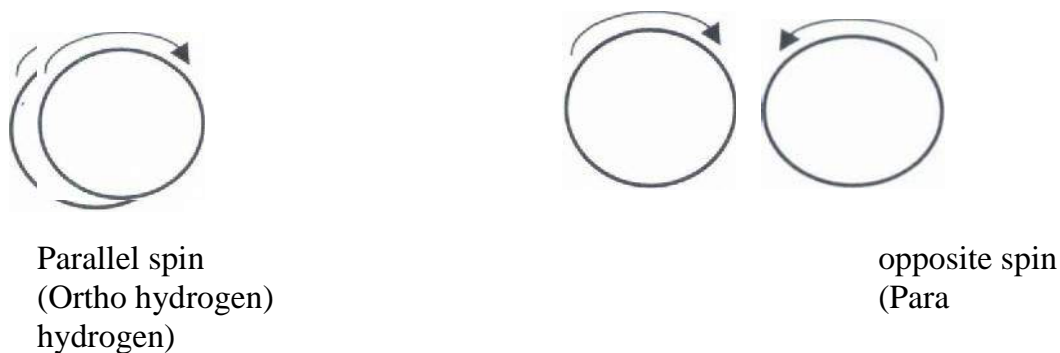
Fig .8: Ortho and Para forms of hydrogen
