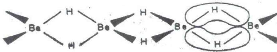
Fig 22: Beryllium hydride polymer
