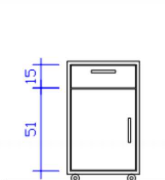
VISTA FRONTAL
