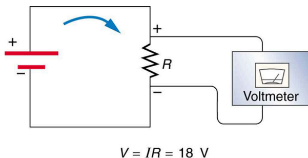
Figure 7.2. The voltage drop across a resistor in a simple circuit equals the voltage output of the battery.
