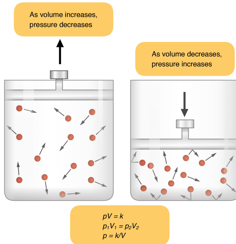
Figure 2.13. Boyle's law. In a gas, pressure increases as volume decreases.
