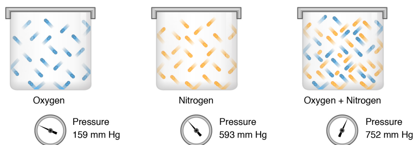
Figure 2.15. Partial pressure is the force exerted by a gas. The sum of the partial pressures of all the gases in a mixture equals the total pressure.
